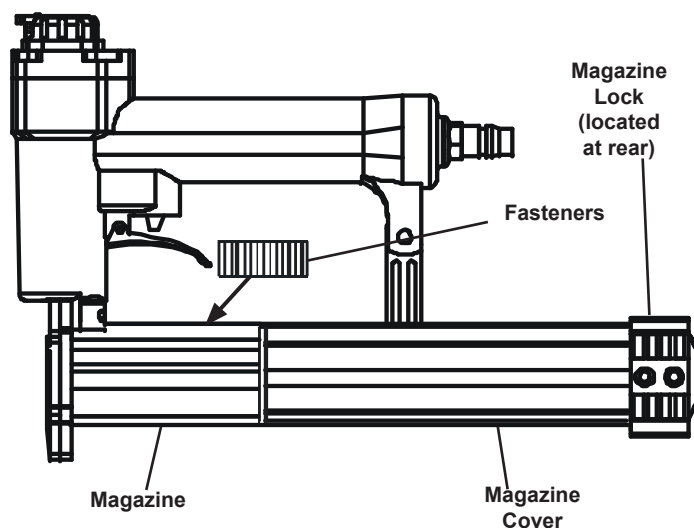
Figure D: Loading the Tool
