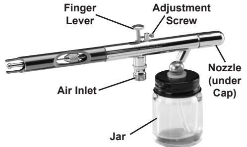
Figure C: Components and Controls
