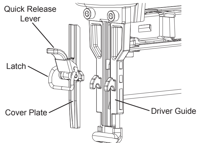
Figure D: Driver Guide and Cover Plate Detail
