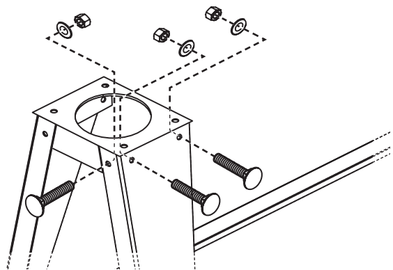
Figure B: Leg Connector Installation
