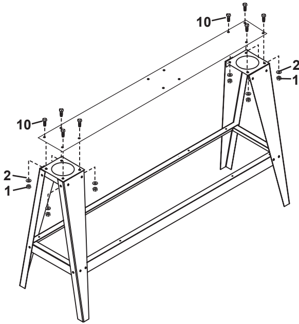
Figure C: Top Installation
