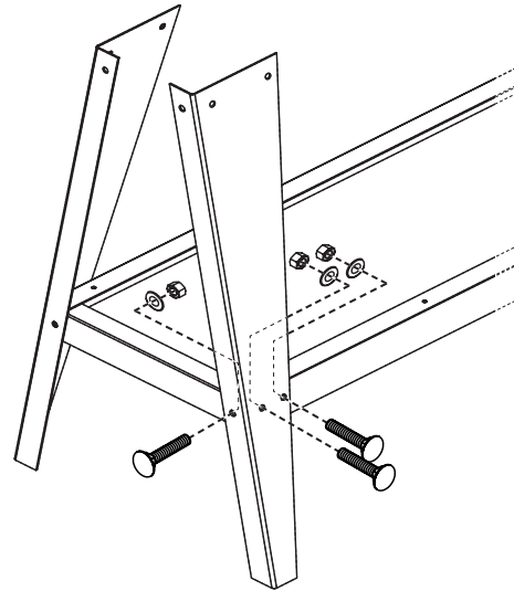
Figure A: Brace Installation
