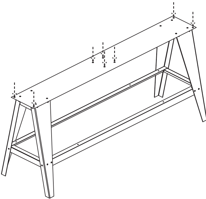
Figure D: Lathe Bolting Locations
