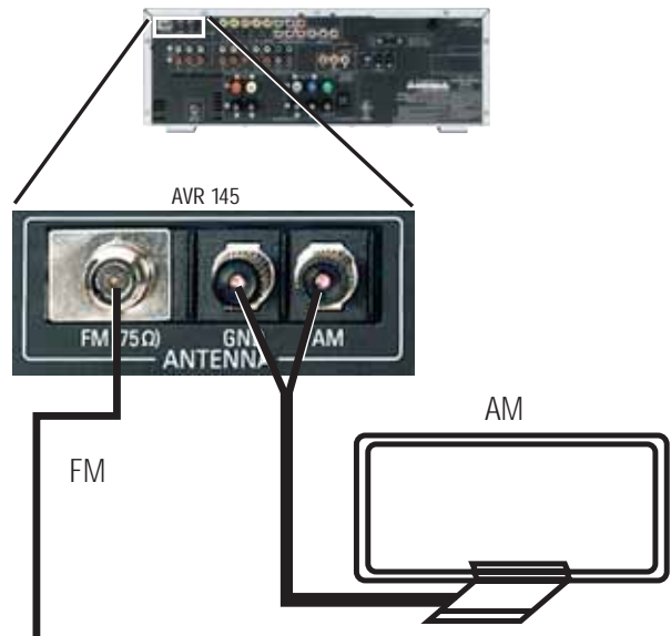
Figure 17 – Antenna Connections
