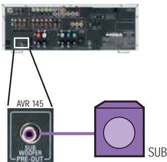
Figure 16 – Subwoofer Connection
