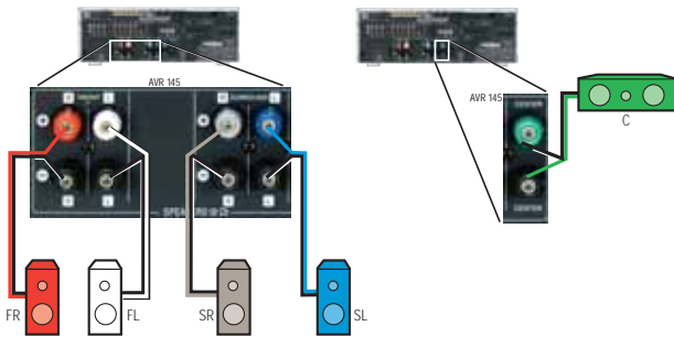
Figure 15 – Speaker Connections
