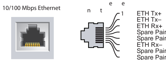
Figure 6 Fast Ethernet Port Pin-Out
