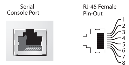
Figure 3 Serial Port Pin-Out
