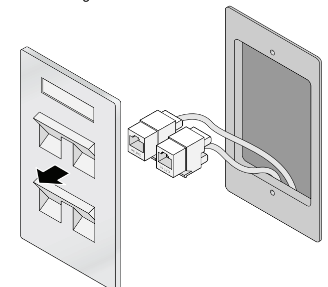
Figure 7 Removing the Wall Plate
