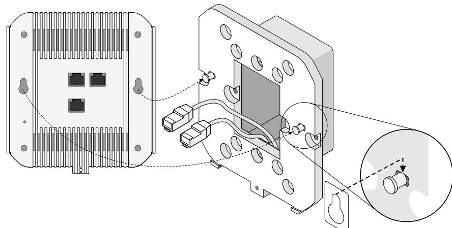
Figure 9 AP-93H to Bracket
