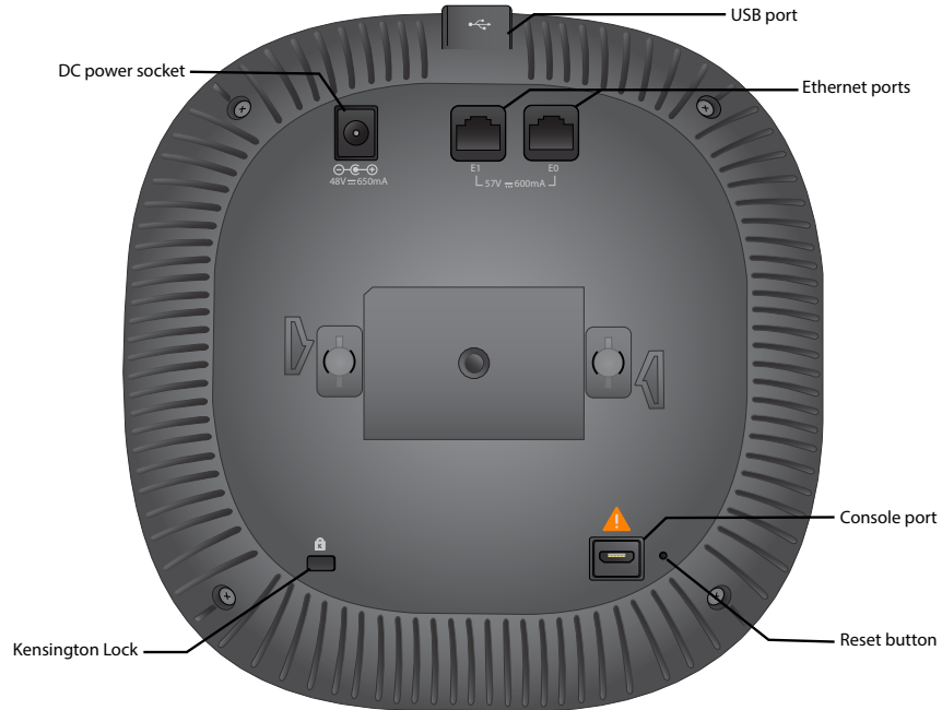
Figure 3 Aruba 340 Series (rear view)
