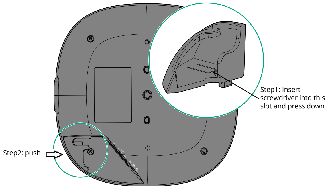
Figure 4 Removing Cable Guide
