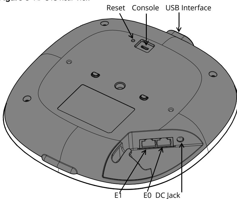
Figure 3 AP-515 Rear View
