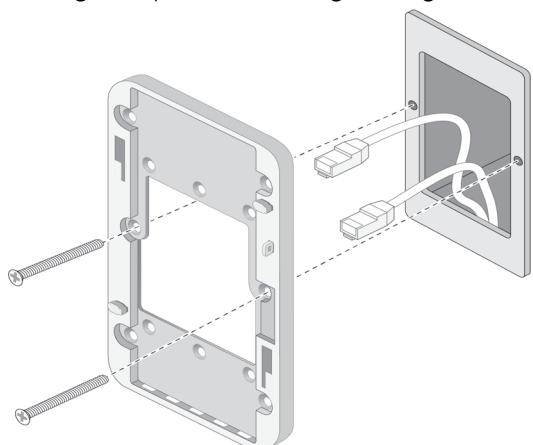
Figure 7 Bracket to Gang Box (Worldwide Single Gang Outlet Box Shown)
