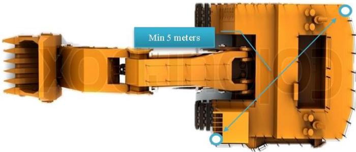
Beacon Antenna
