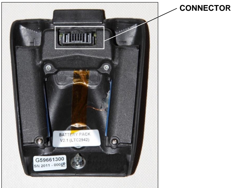
Figure 8 Battery pack
