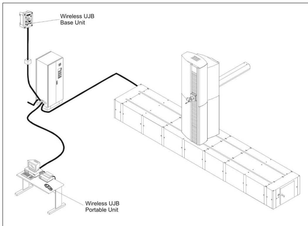
Figure 1 UJB Kit
