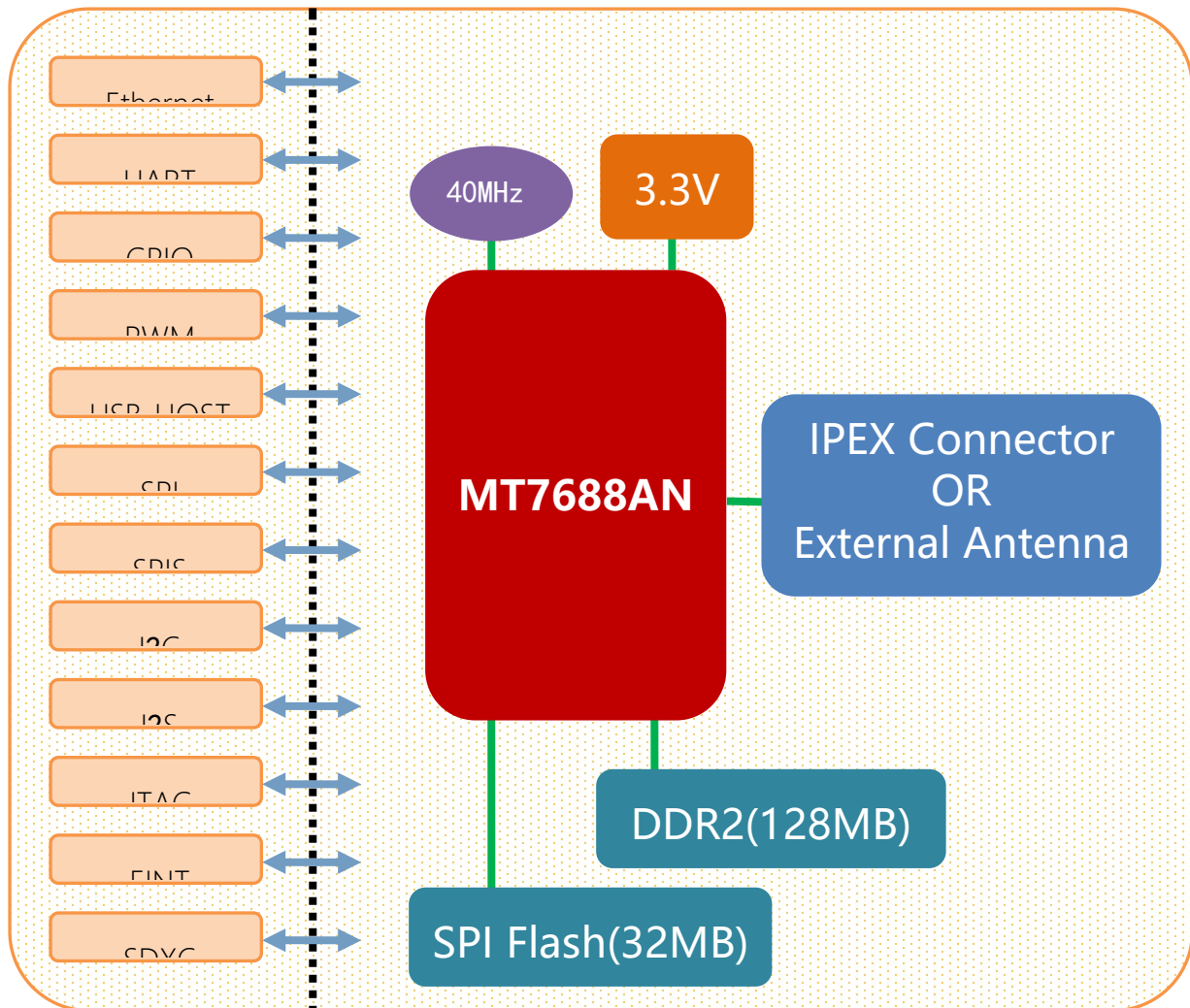
HLK-7688 structure
