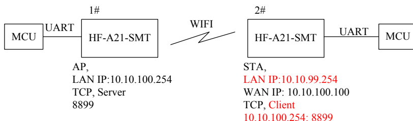
Figure 42. Configure Transparent Serial Port Connection (TCP)
