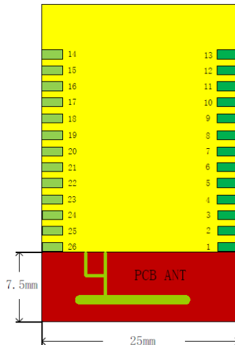
Figure 4. HF-A21-SMT Chip Antenna Keep Out Region
