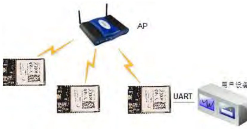
Figure 15. HF-A21-SMT Basic Wireless Network Structure
