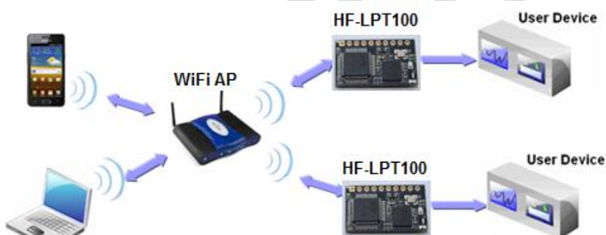
Figure 8. HF-LPT100 Basic Wireless Network Structure
