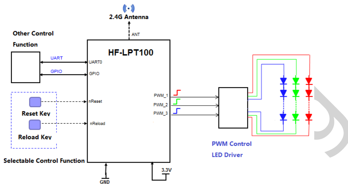
Figure 7. HF-LPT100 Smart LED Application Hardware Connection
