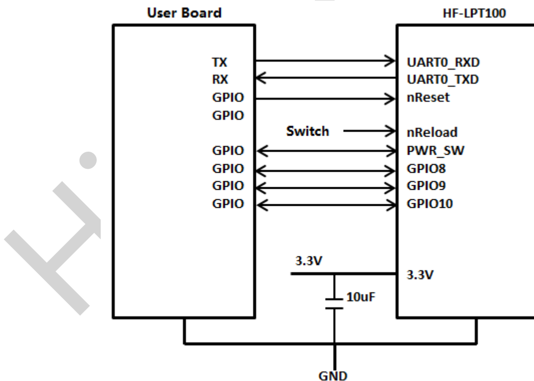
Figure 6. HF-LPT100 Hardware Typical Application
