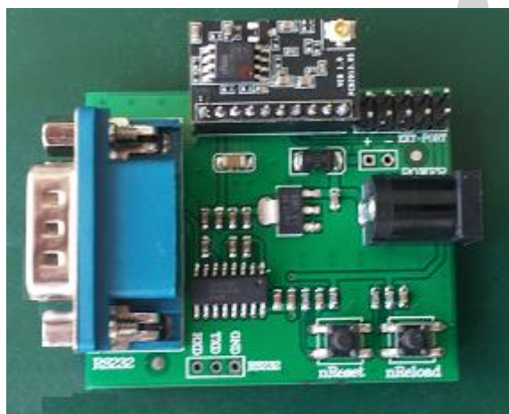
Figure 4. HF-LPT100 Evaluation Kit
