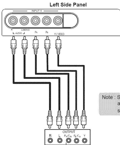
COMPONENT OUTPUT CAPABILITY DVD , Set Top Box, Video Game Console.
