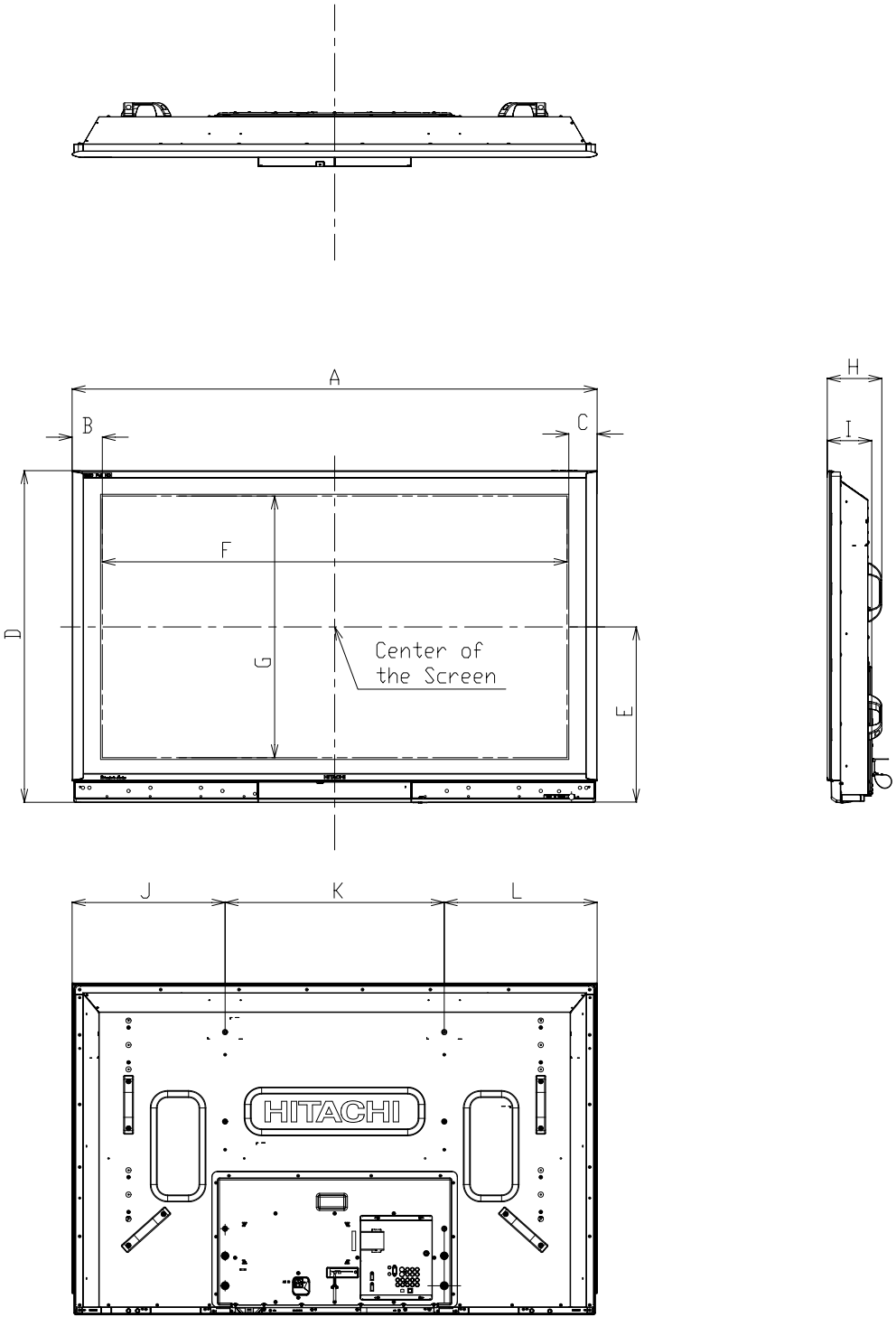
Rear View, Use as Reference for Wall Mount Bracket
