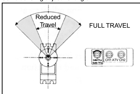
Servo traveling adjustment fig 5
