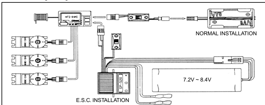
Installation diagram fig 7
