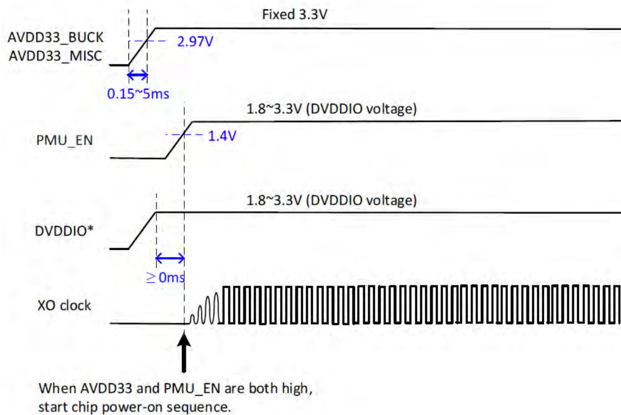
Figure 2 Power Sequence
