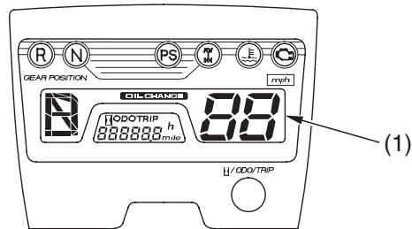
(1) multi-function display
