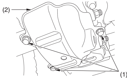
(1) skid plate bolts (2) skid plate
