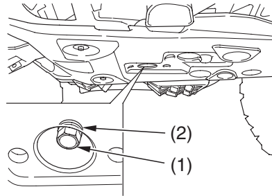
(1) engine oil drain bolt (2) sealing washer
