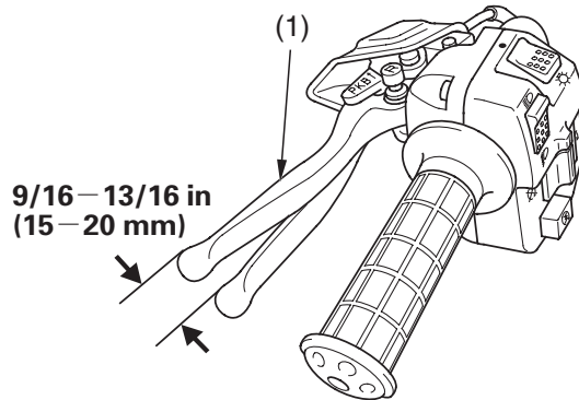
(1) rear brake lever/parking brake lever
