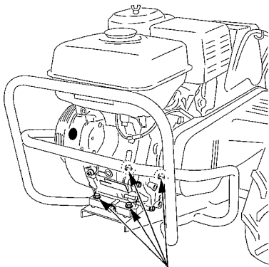
ENGINE MOUNTING BOLTS
