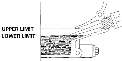
ENGINE OIL FILLER CAP/DIPSTICK
