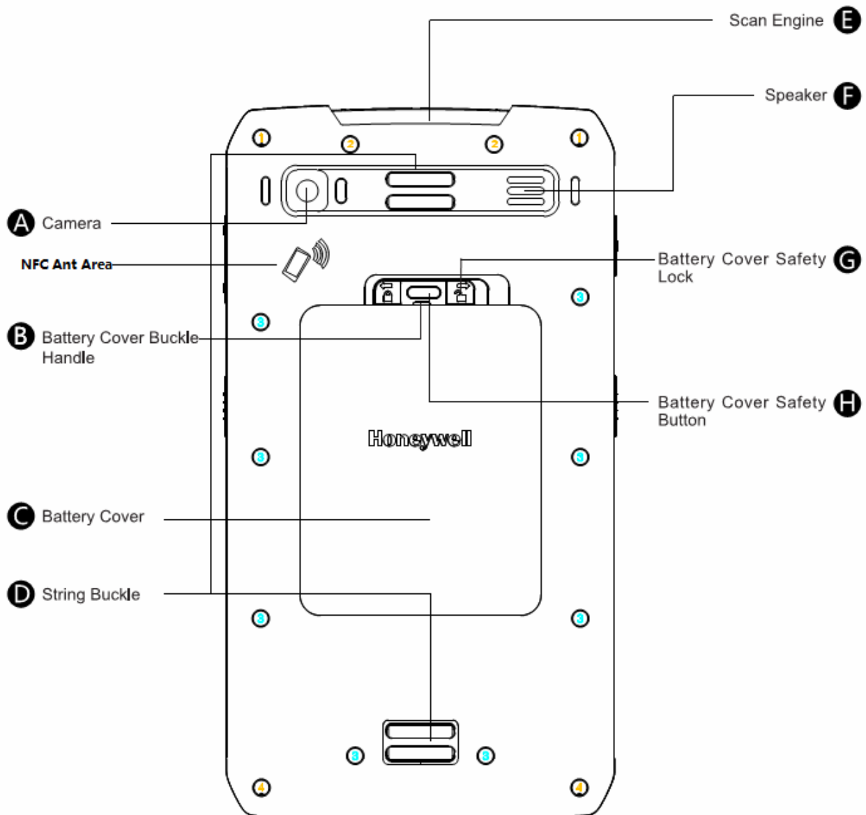
Back view of the EDA70-3
