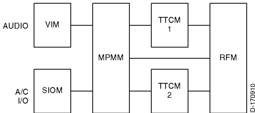
Figure 1-5. MCS-7200 SDU Equipment Description
