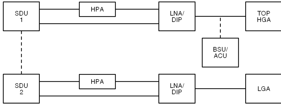
Figure 2-3. HGA + LGA Configuration with Top-Mounted HGAs
