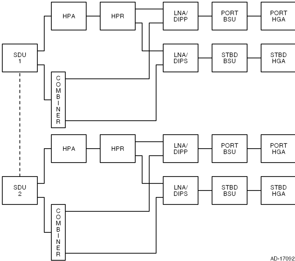
Figure 2-6. HGA + HGA Configuration with Two Side-Mounted HGAs
