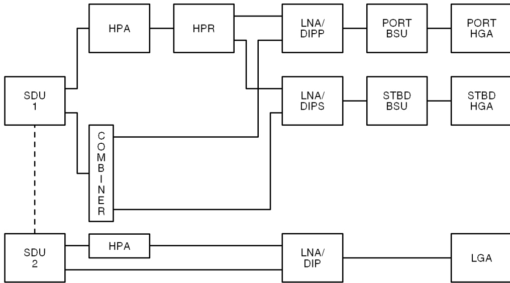
Figure 2-4. HGA + LGA Configuration with Side-Mounted HGAs
