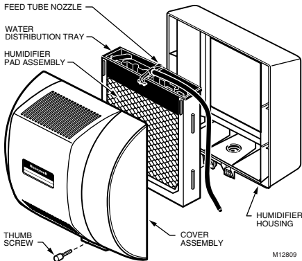
Fig. 3. Disassembling humidifier.
