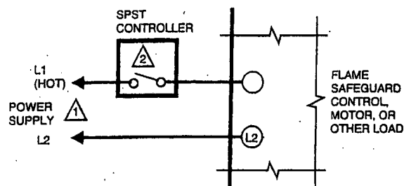
Fig. 5—L404 used as a limit or as an operating controller.
