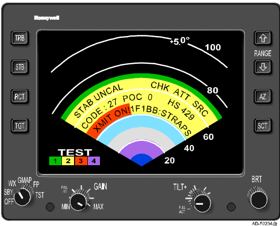
Radar Indication With Text Fault Enabled (On Ground) Figure 7- 3
