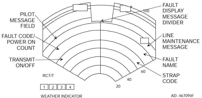
Fault Annunciation on Weather Indicator With TEXT FAULT Fields Figure 7- 1
