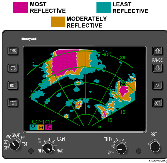
Ground Mapping Display Figure 5- 49
