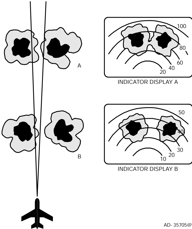
Azimuth Resolution in Weather Modes Figure 5- 40
