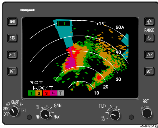
Typical PRIMUS® 880 Digital Weather Radar Display Figure 3- 1
