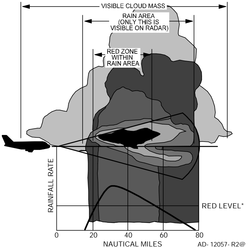
Radar and Visual Cloud Mass Figure 5- 26
