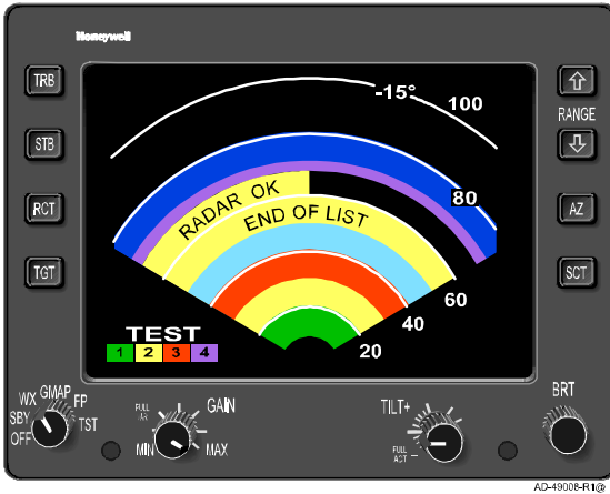
WI-880 Indicator Test Pattern With TEXT FAULT Enabled Figure 4-3
