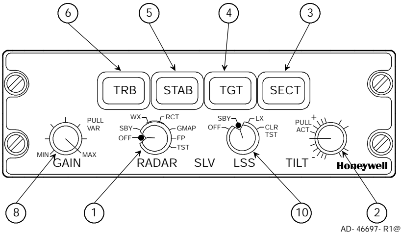
WC- 880 Weather Radar Controller Configurations Figure 3- 4
