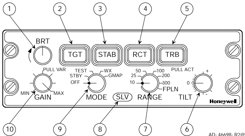
WC- 884 Weather Radar Controller Figure 3- 5
