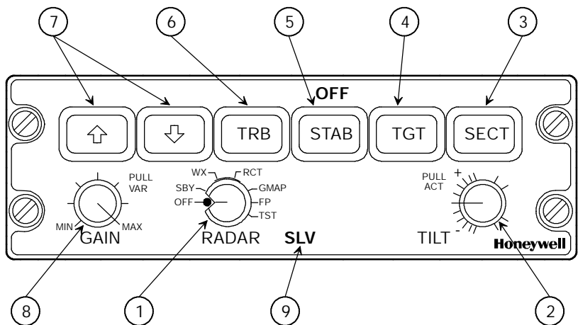
WC- 880 Weather Radar Controller Configurations Figure 3- 4 (cont)
