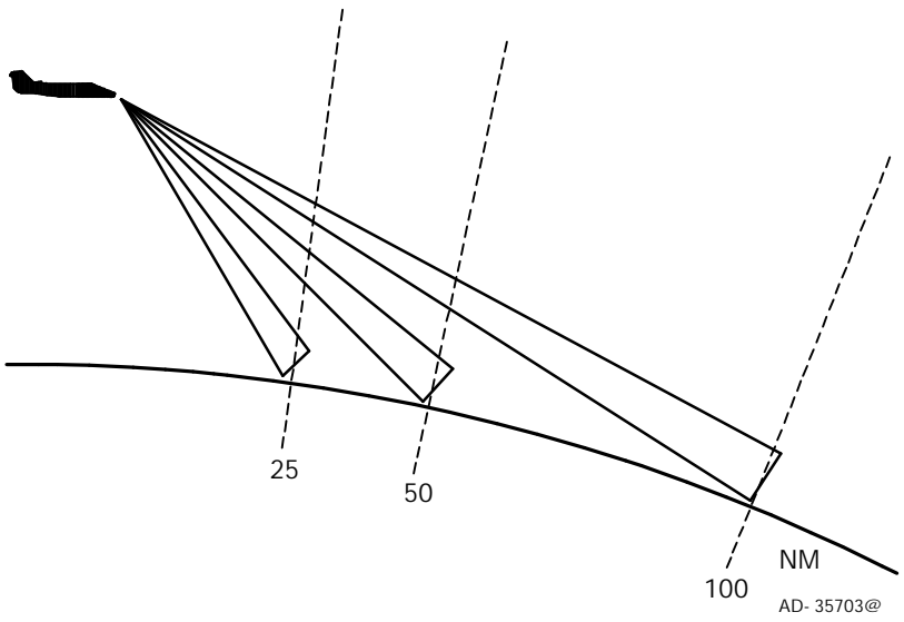
Manual Tilt at Low Altitudes Figure 5- 18
