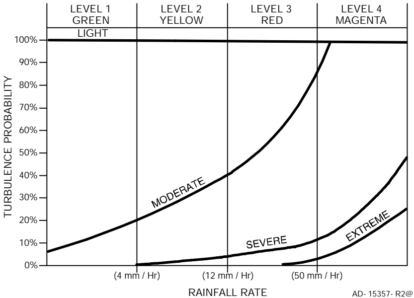
Probability of Turbulence Presence in a Weather Target Figure 5- 29
