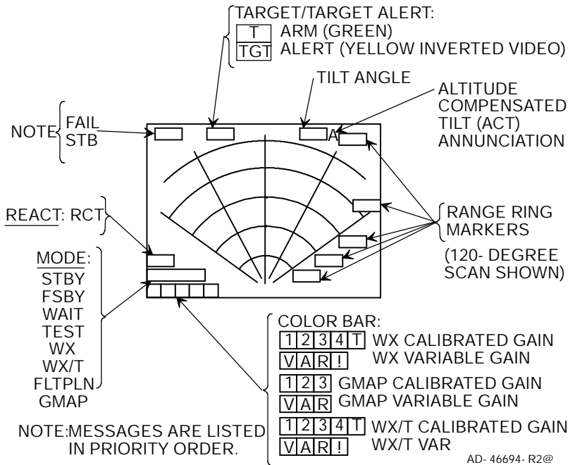
WI- 880 Weather Radar Indicator Display Screen Features Figure 3- 3
