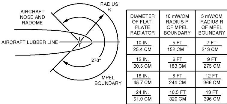
MPEL Boundary Figure 6-1
