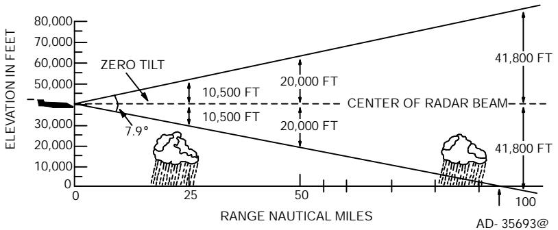
Radar Beam Illumination High Altitude 12- Inch Radiator Figure 5- 4
