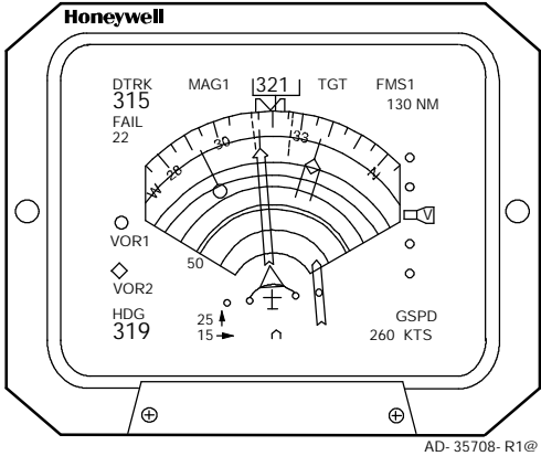
Fault Code on EFIS Weather Display With TEXT FAULTS Disabled Figure 7- 2
