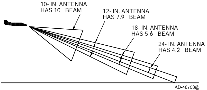
Antenna Size and Impact on Tilt Management Figure 5- 16
