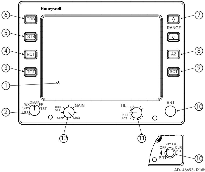
WI- 880 Weather Radar Indicator Front Panel View Figure 3- 2
