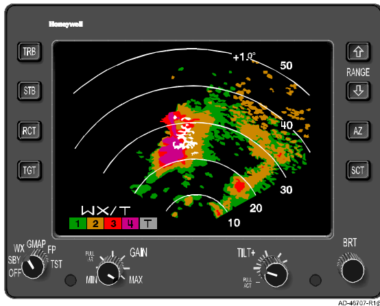
Weather Display With Turbulence Figure 5- 33
