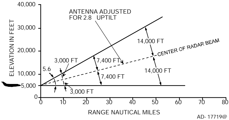
Radar Beam Illumination Low Altitude 18- Inch Radiator Figure 5- 7
