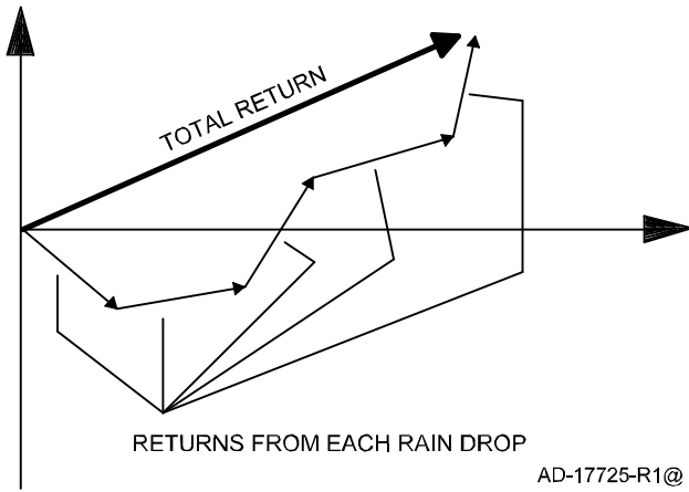
Total Return Vector Figure 5- 30
