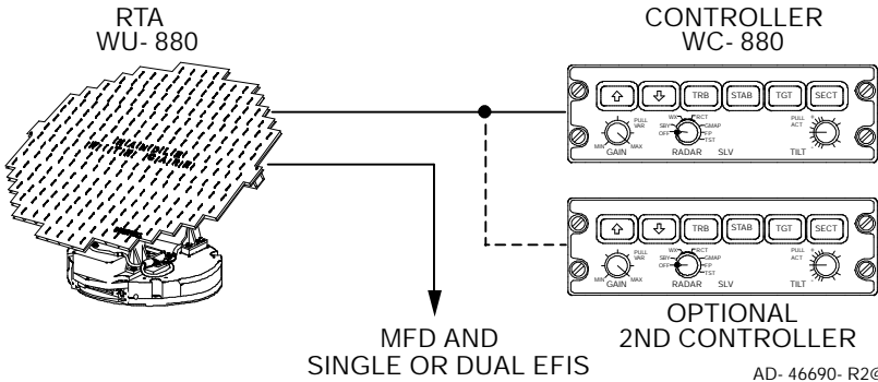
PRIMUS ® 880 Configurations Figure 2- 1
