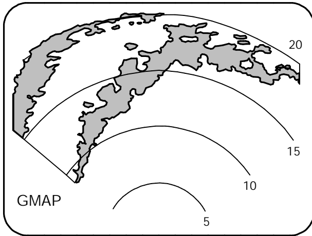
Ground Return Indicating Misalignment (Upper Left) Figure 5- 21
