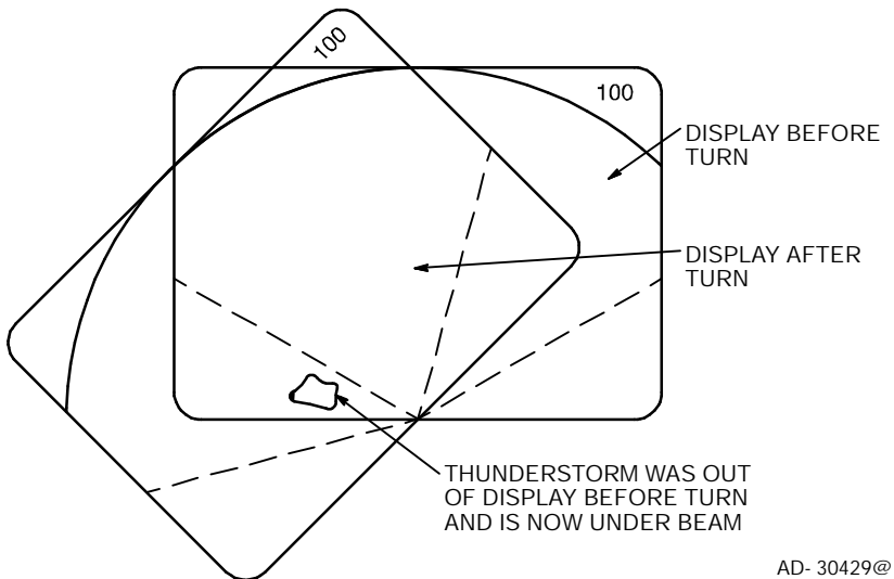
Tilt Management With Heading Changes Figure 5- 13
