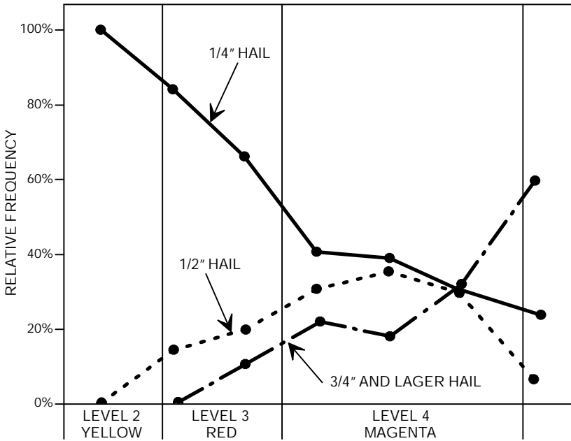
Hail Size Probability Figure 5- 35
