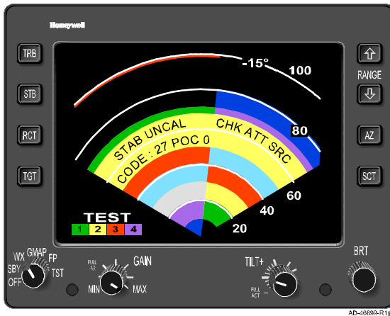
Indicator Test Pattern 120° Scan (WX), With TEXT FAULT Enabled Figure 4- 1
