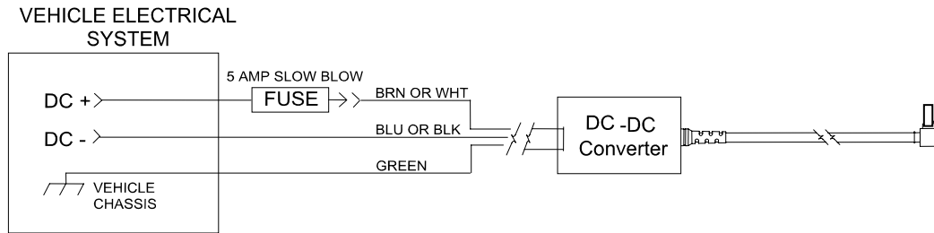
Figure 17 Connecting the Power Supply to the MX3P Endcap Power Jack
