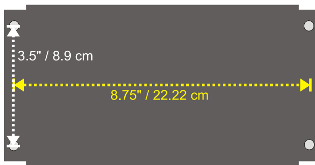
Figure 18 Vehicle Power Supply Footprint
