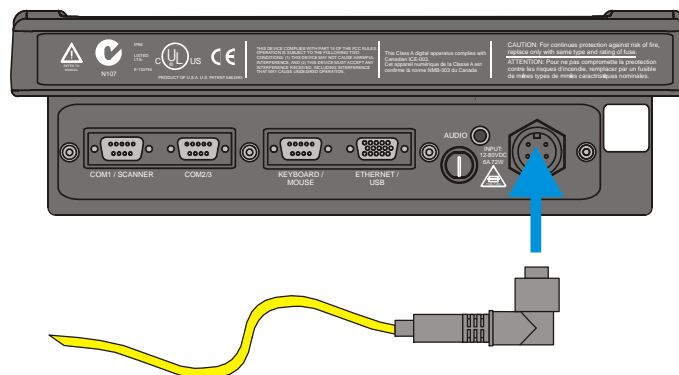
Figure 60 Connect Power Cable to VX7
