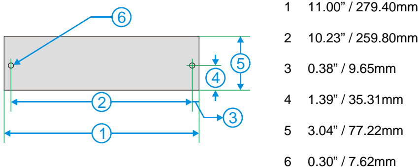
Figure 46 UPS Battery Pack Remote Mounting Dimensions
