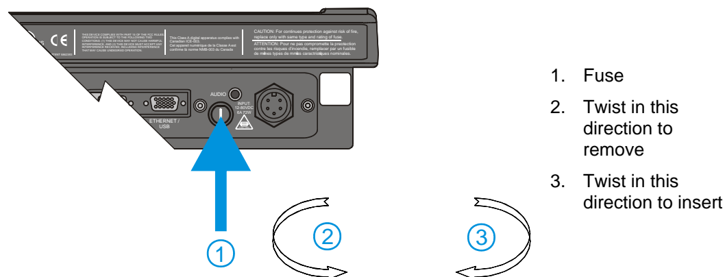
Figure 69 Fuse Replacement
