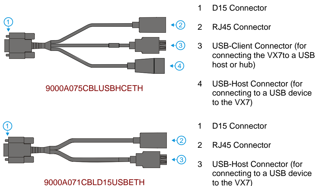
Figure 55 VX7 Ethernet/USB-H/USB-C Dongle Cables
