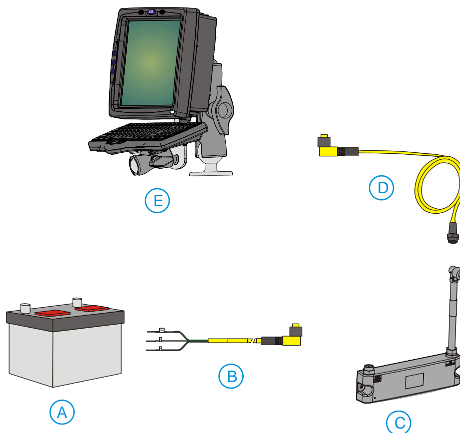
Figure 67 Remote Mount UPS Battery Pack Connection
