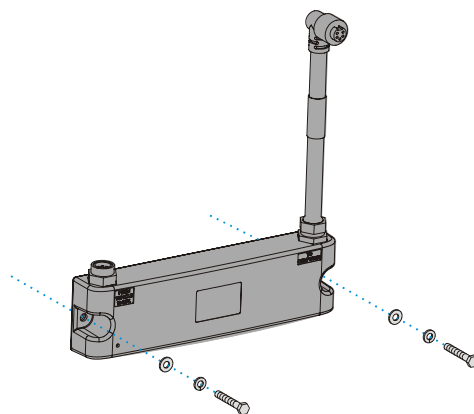
Figure 45 Remote UPS Battery Pack Mount
