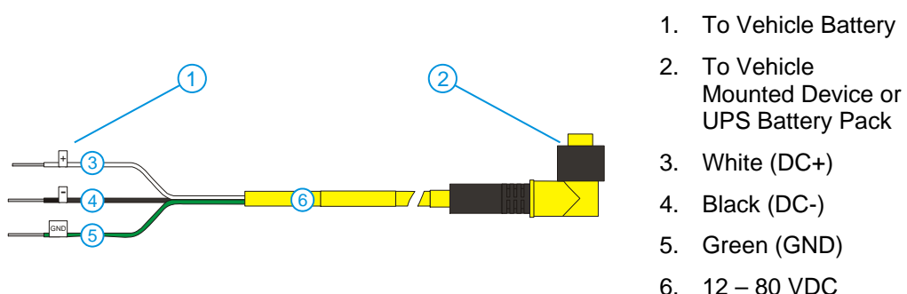
Figure 62 Vehicle Power Connection Cable (Fuse Not Shown)
