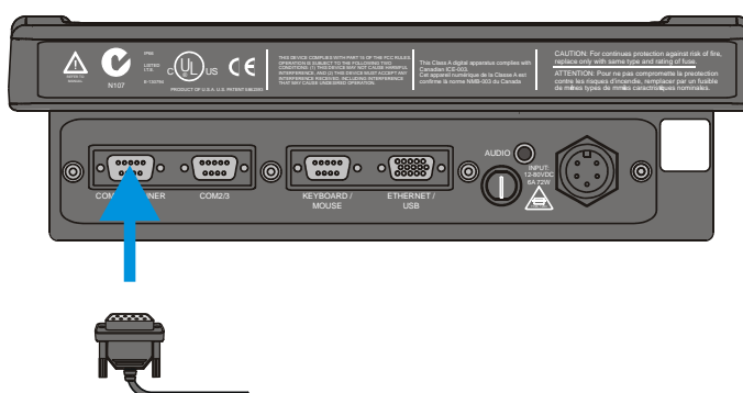
Figure 51 Connect Serial Scanner Cable
