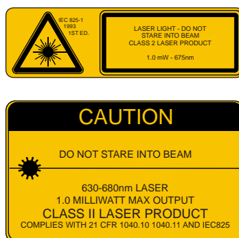
Figure 74 Caution Labels Class II Scanner
