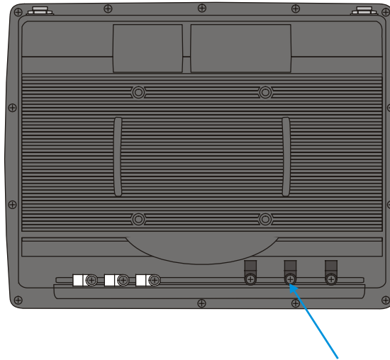
Figure 70 Strain Relief Cable Clamps
