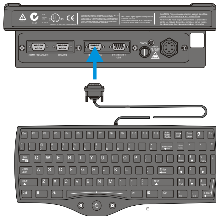
Figure 47 Keyboard Connection Location and Keyboard
