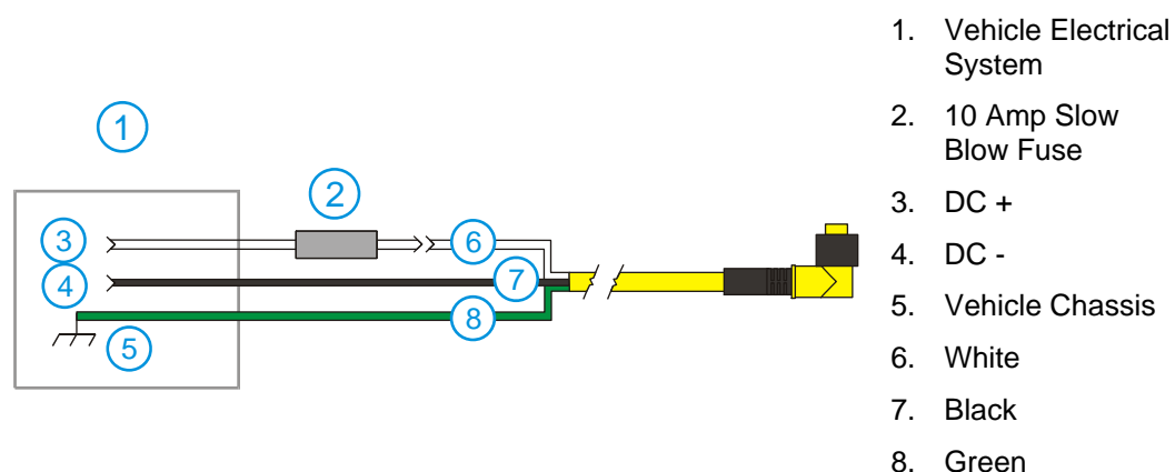
Figure 63 Connecting the Power Cable to the Vehicle
