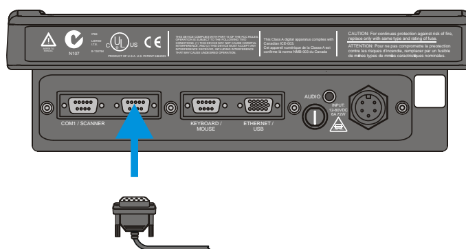
Figure 54 Connect Serial Cable to COM3
