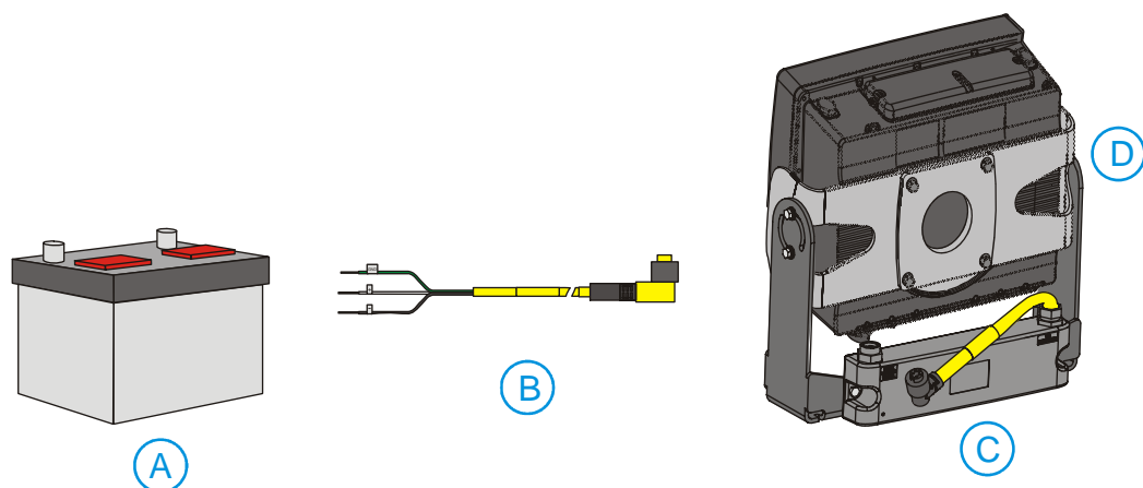
Figure 66 Integrated Mount UPS Battery Pack Connection
