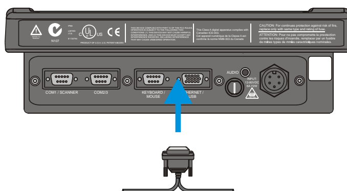
Figure 56 Connect Ethernet/USB Dongle Cable
