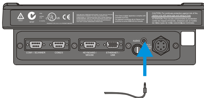
Figure 59 Connect External Headset
