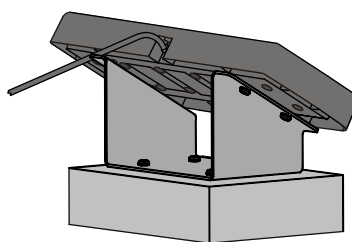
Figure 43 Remote Keyboard Bracket Assembly
