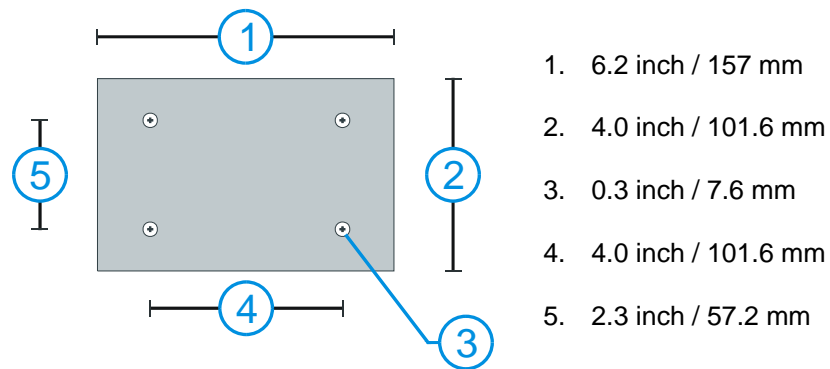
Figure 44 Remote Keyboard - Mounting Dimensions
