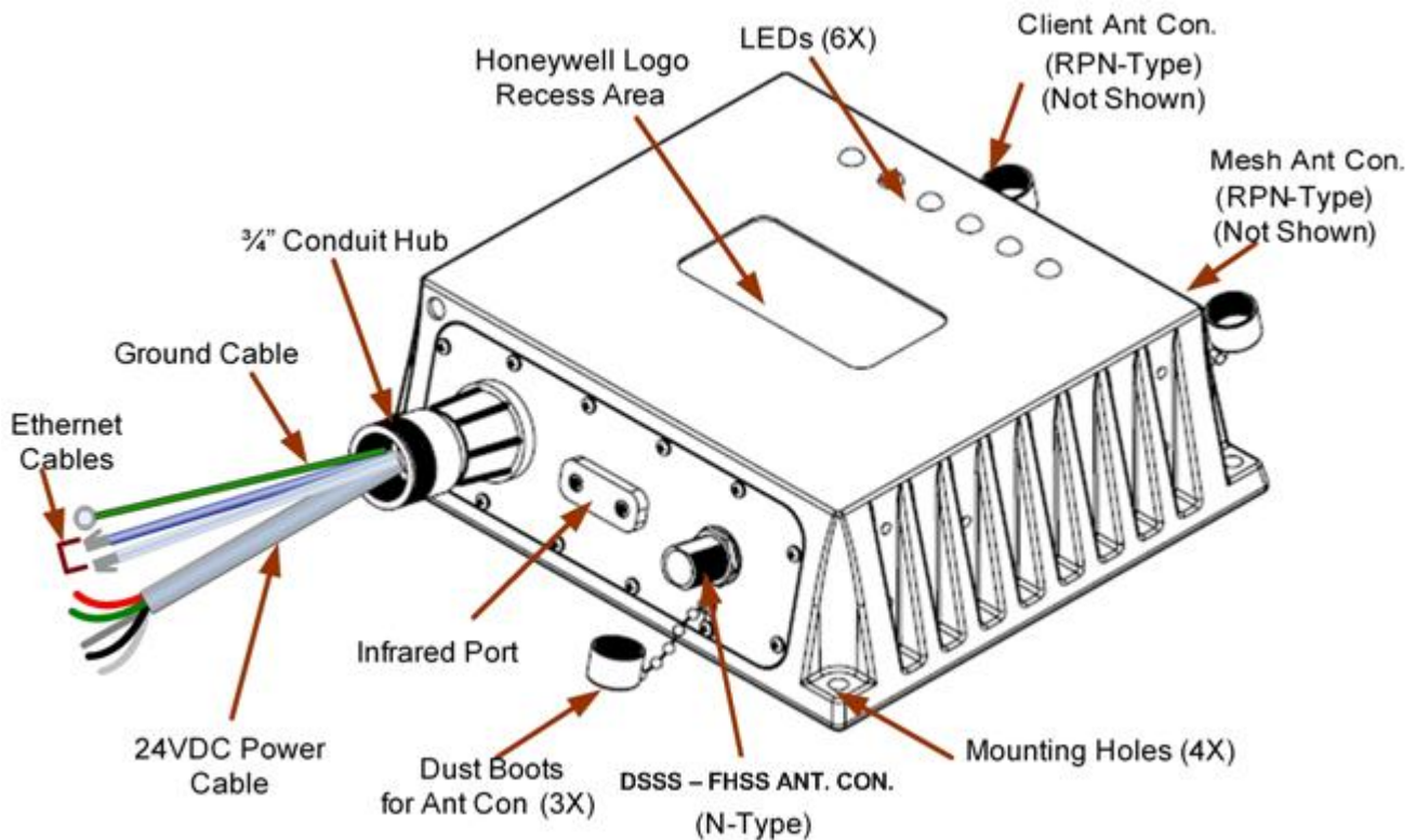
Figure 1 –Diagram of Multinode Unit showing various external attributes
