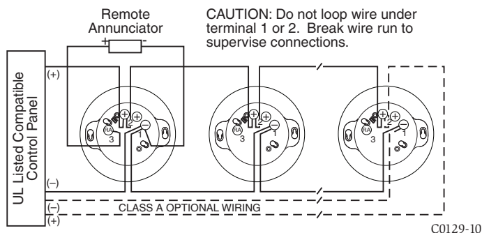
FIGURE 2. WIRING DIAGRAM
