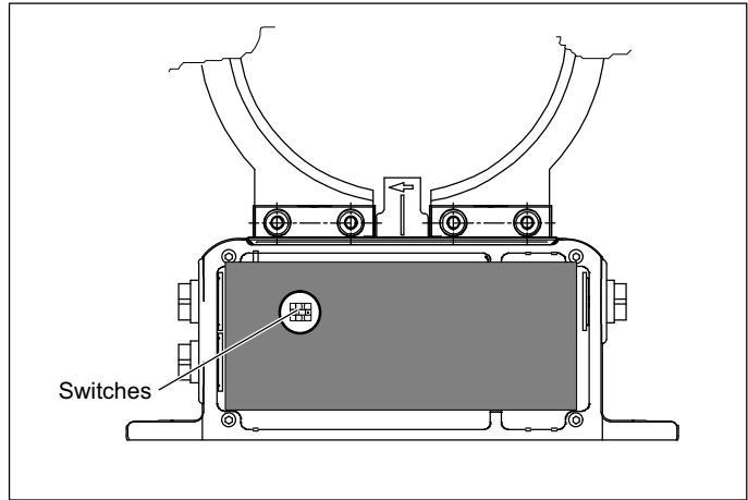
Fig. 7.3 Switches in the stator housing
