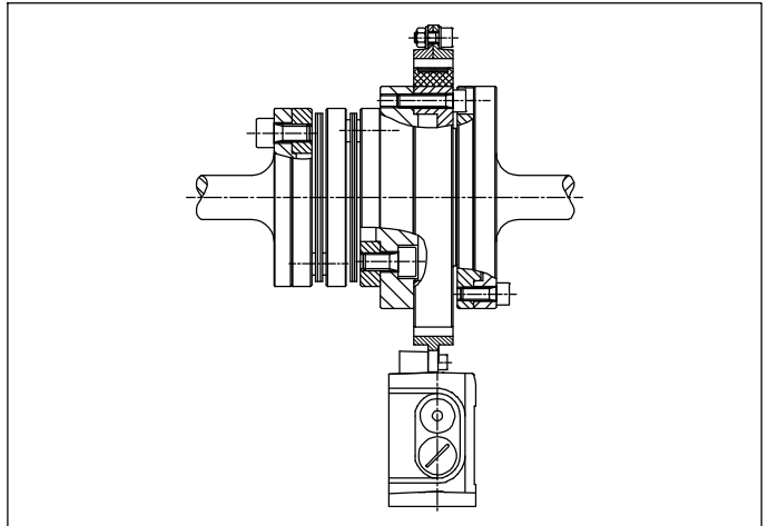
Fig. 6.1 Installation example with coupling
