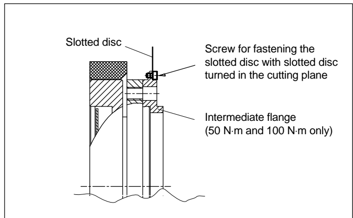
Fig. 6.8 Installing the slotted disc
