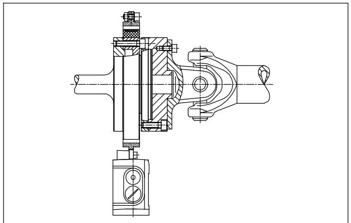
Fig. 6.2 Installation example with joint shaft
