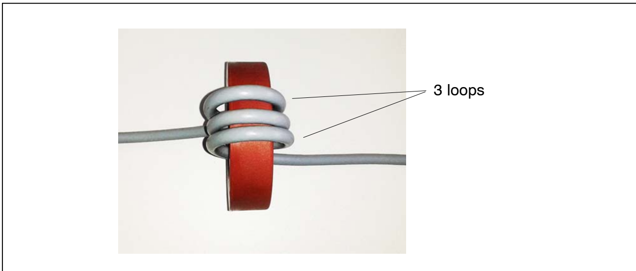
Fig. 6.21: Installation Example
