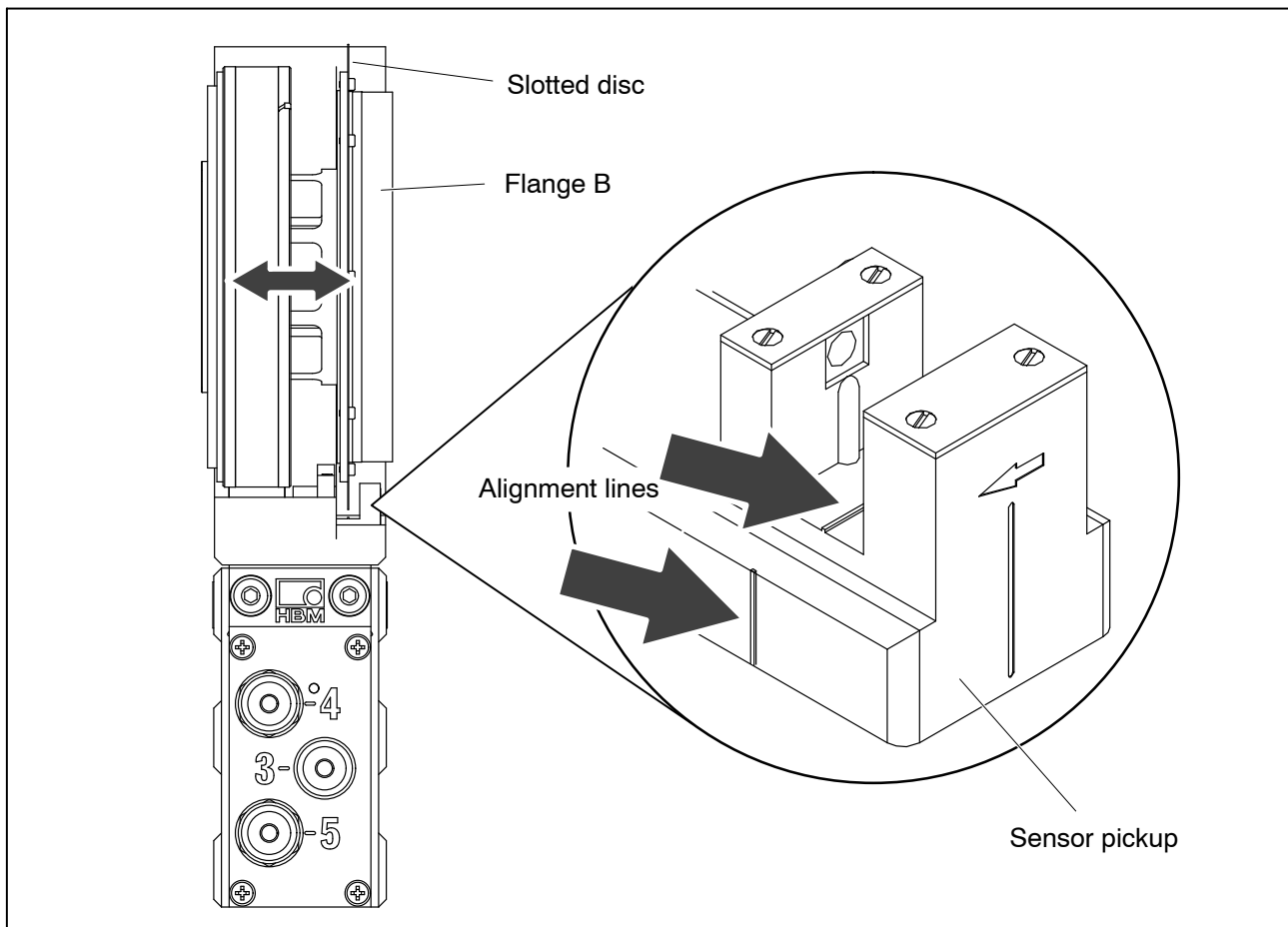
Fig. 6.19: Position of the slotted disc in the rotational speed sensor
