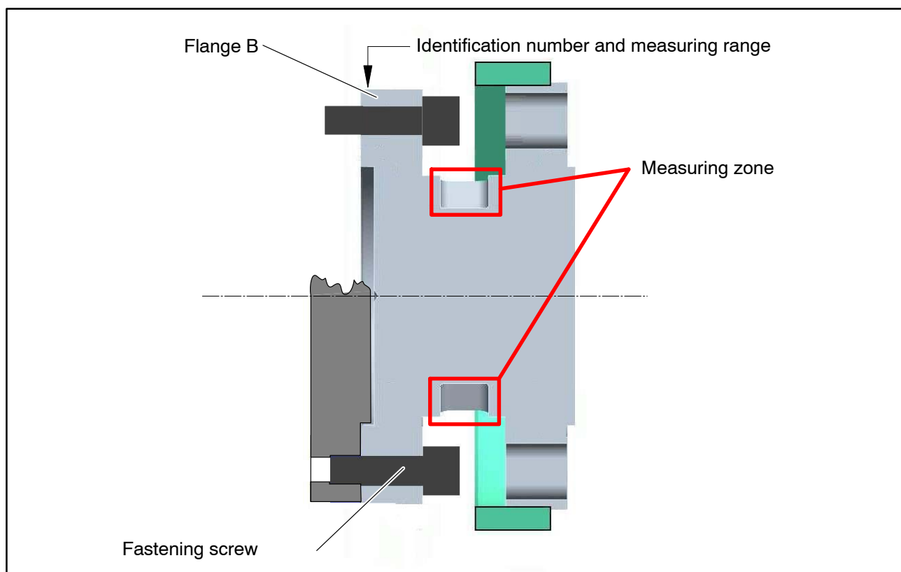
Fig. 6.2: Screw connections, flange B
