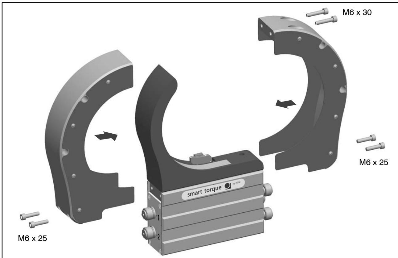
Fig. 6.9: Fit the protection against contact halves
