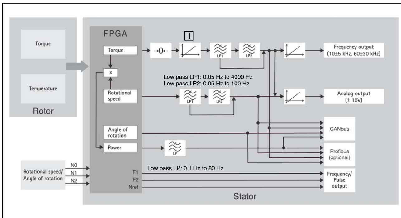
Fig. 4.1: Signal flow diagram
