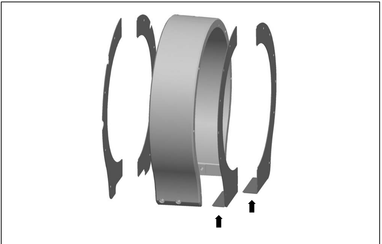
Fig. 6.8: Angled cover plates (5 kN·m and 10 kN·m measuring ranges)
