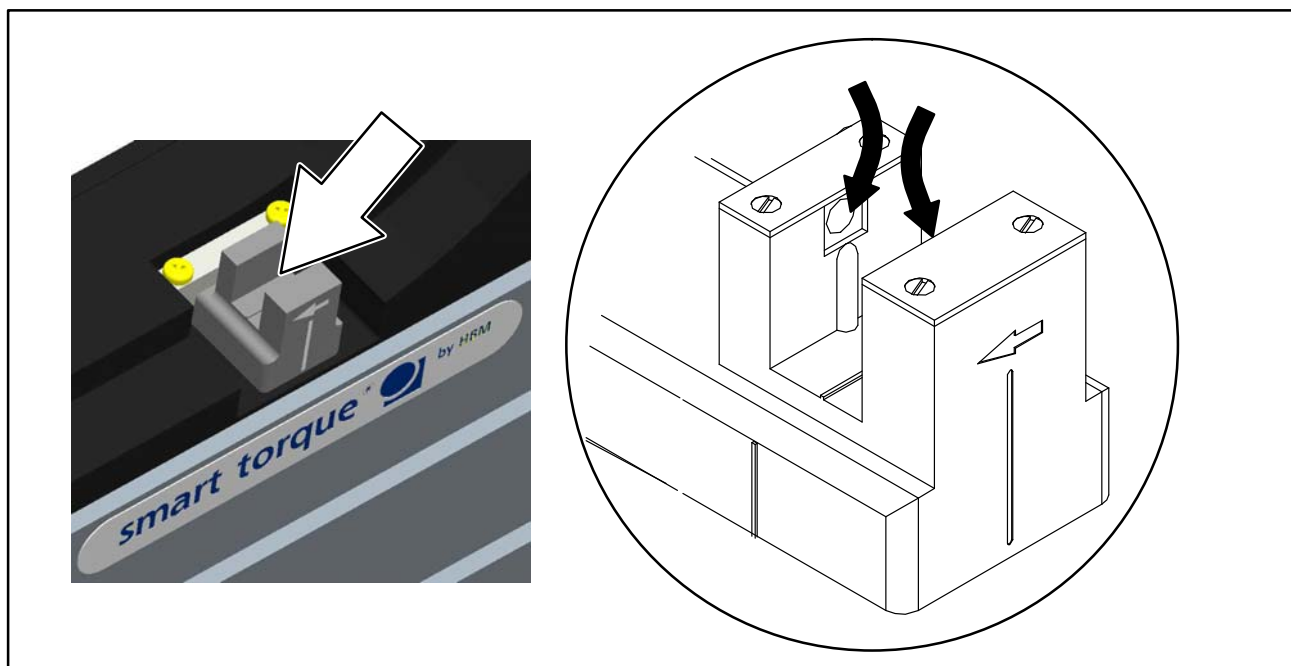
Fig. 12.1: Cleaning points on the rotational speed sensor
