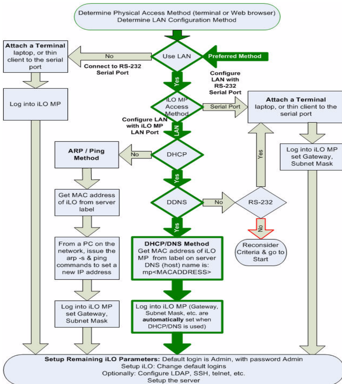
Figure 3-1 Setup Flowchart
