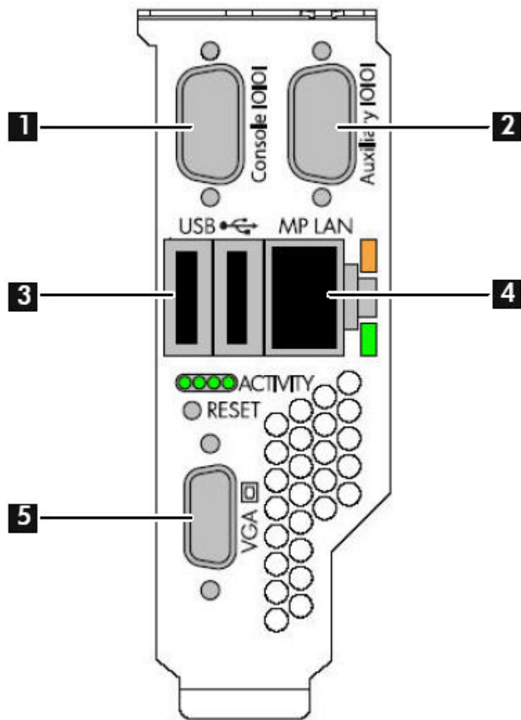
Figure 2-4 HP Integrity rx3600 and rx6600 Server Rear Ports and LEDs
