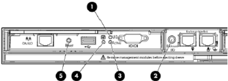
Figure 2-2 Onboard Administrator LEDs and Buttons
