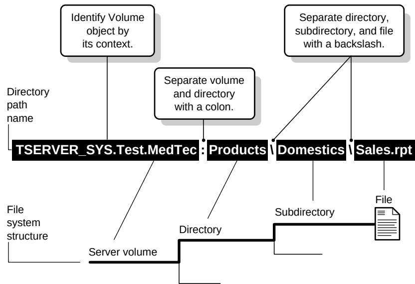
Figure 1-5 NetWare 4 File System Structure and Directory Path
