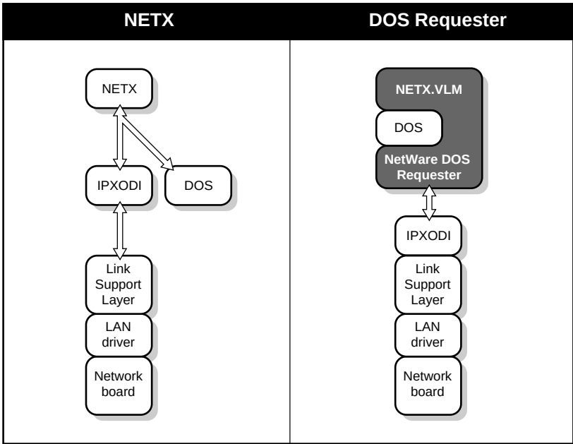
Figure 2-3 Comparison of NETX and NetWare DOS Requester Architecture
