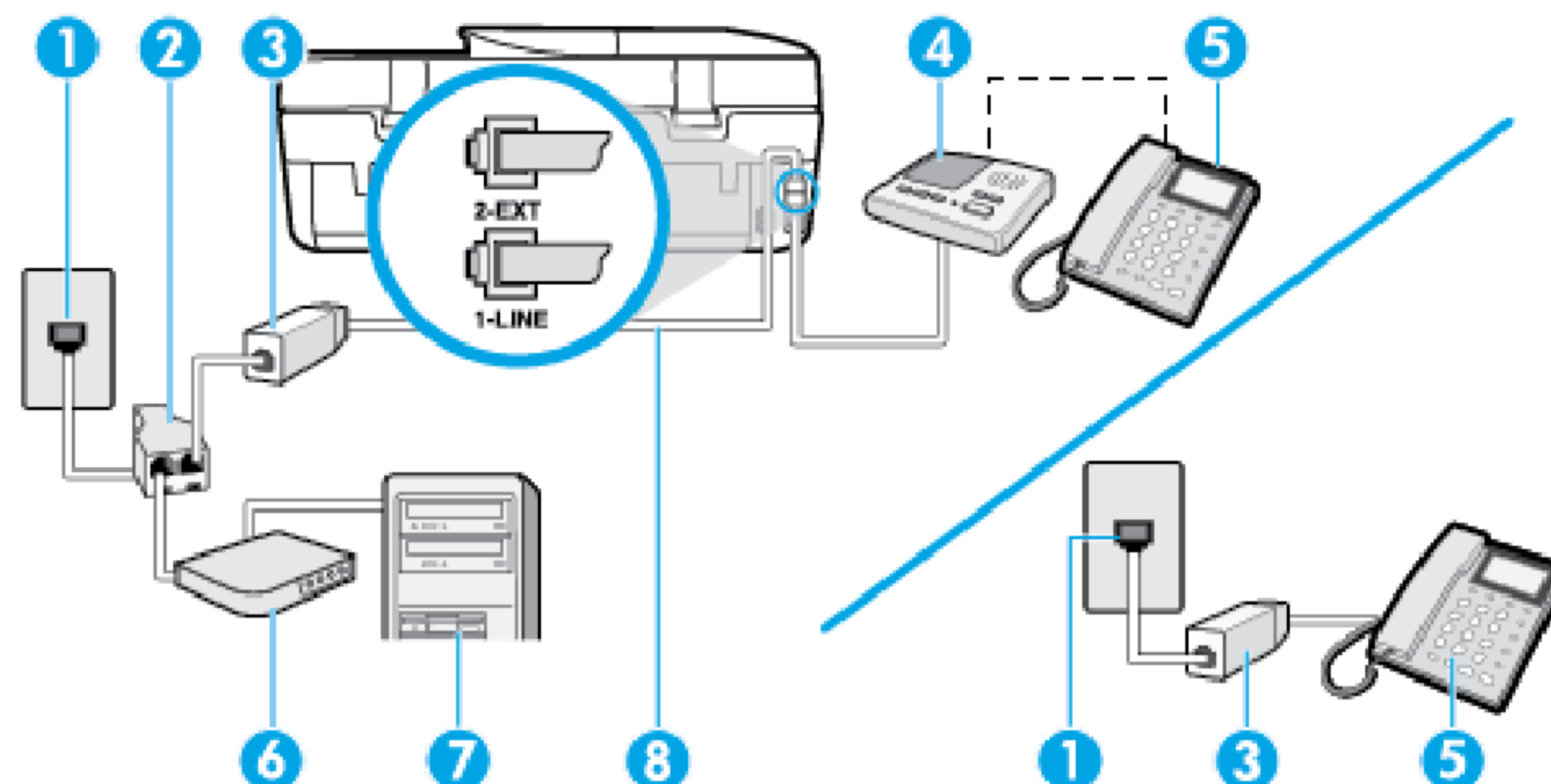
Figure B-15 Back view of the printer
