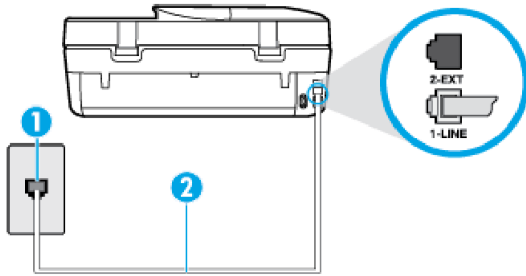
Figure 9-1 Back view of the printer
