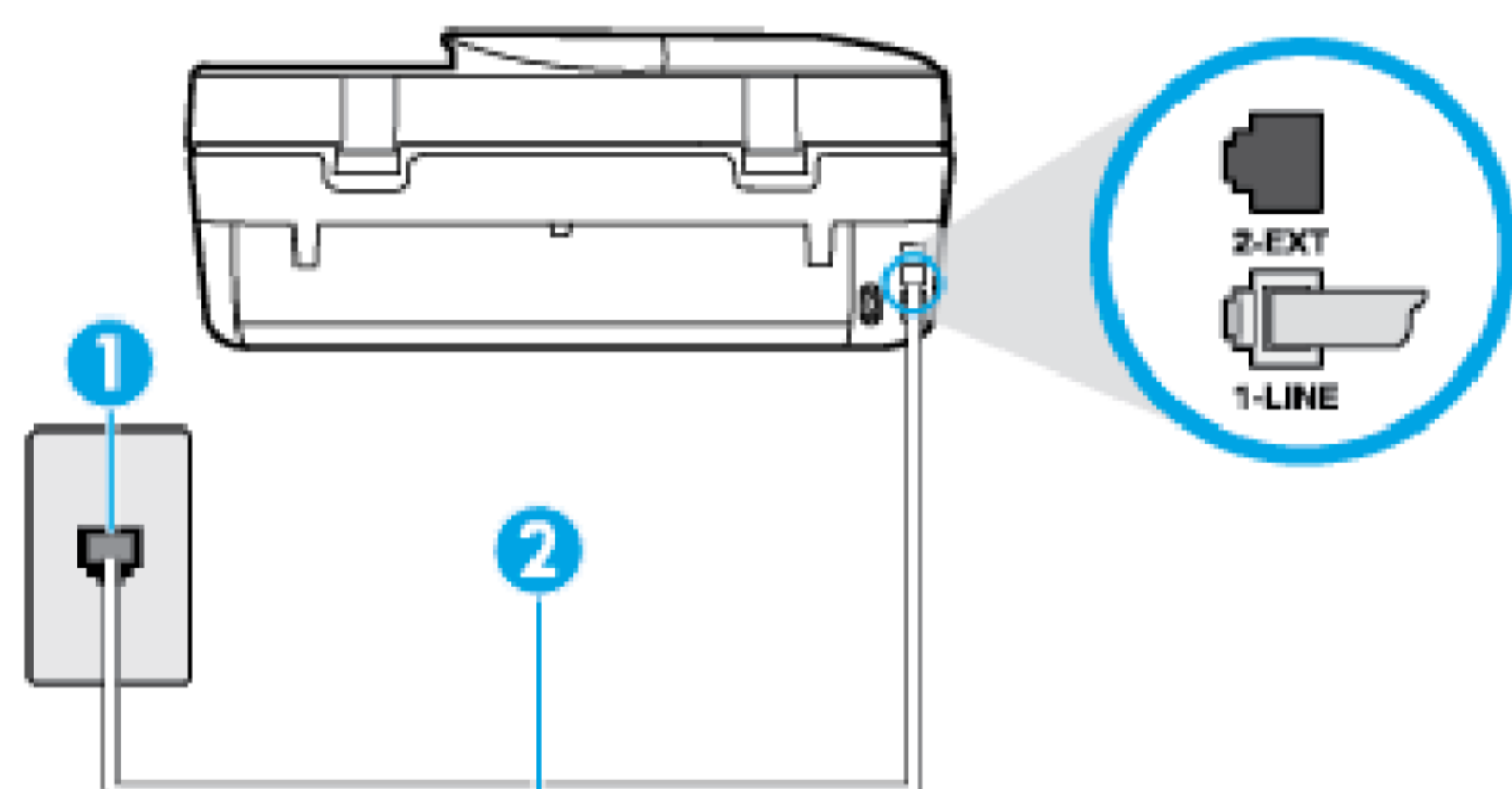
Figure B-5 Back view of the printer
