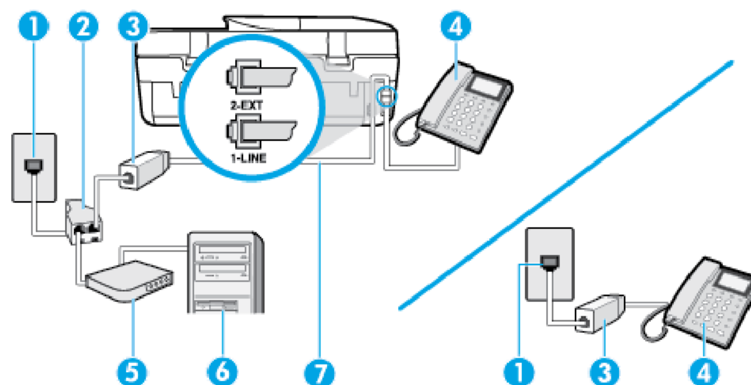
Figure B-10 Back view of the printer
