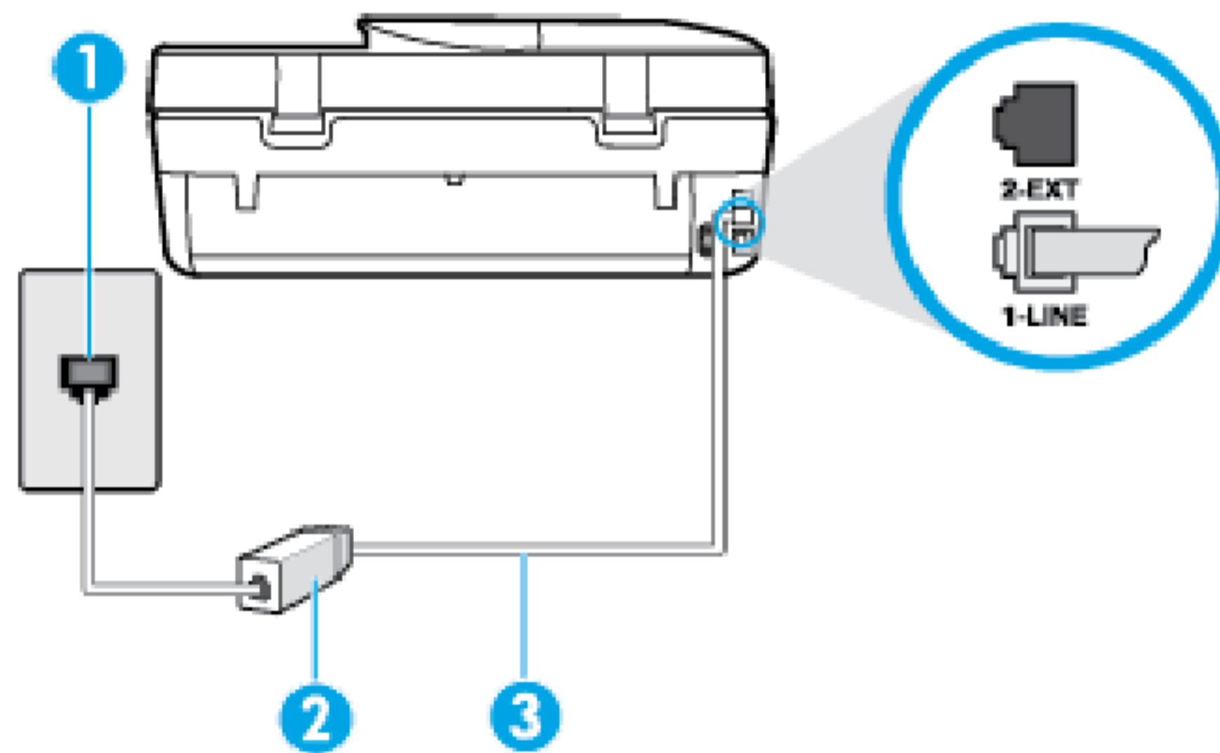
Figure B-2 Back view of the printer
