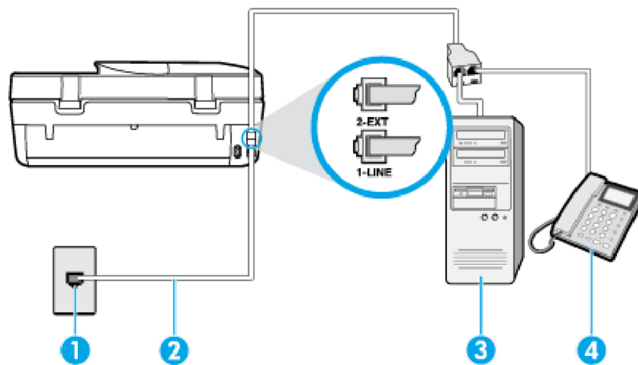
Figure B-18 Back view of the printer
