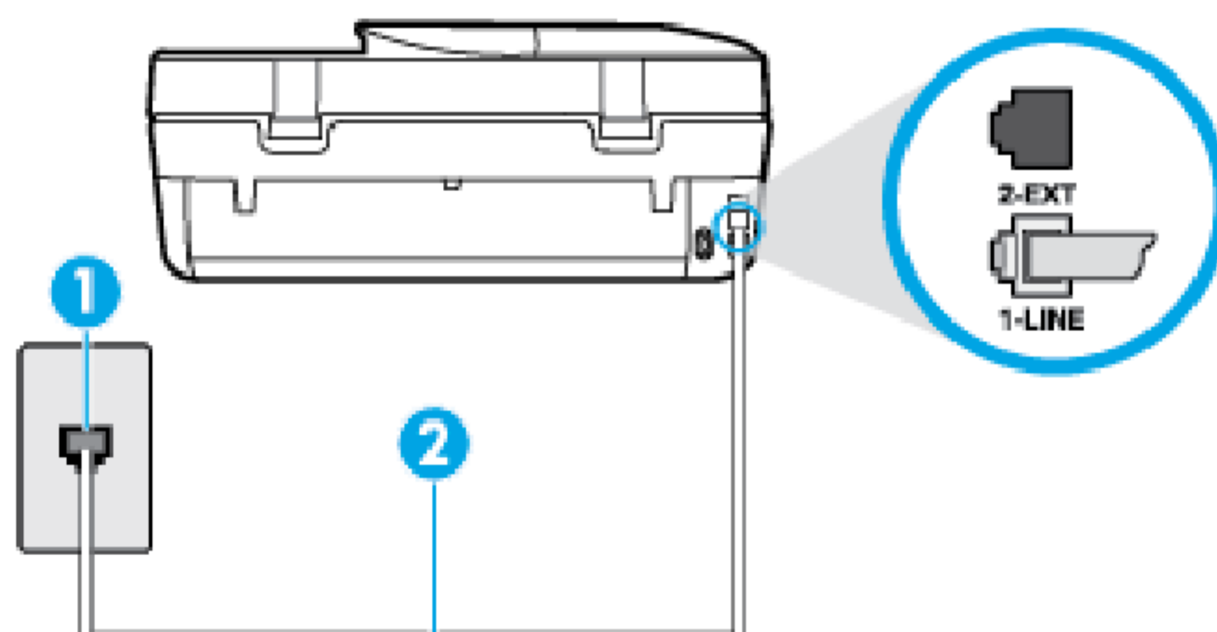
Figure B-3 Back view of the printer
