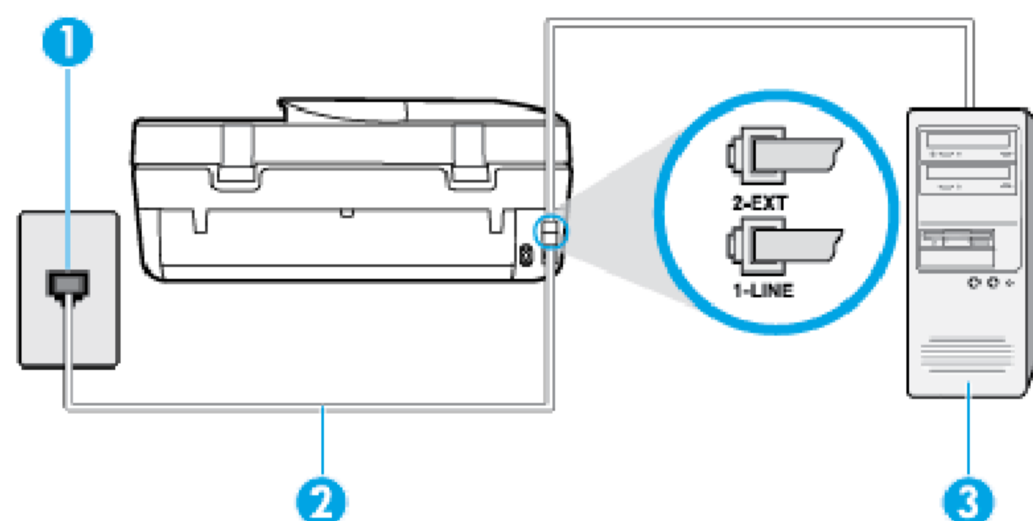
Figure B-6 Back view of the printer
