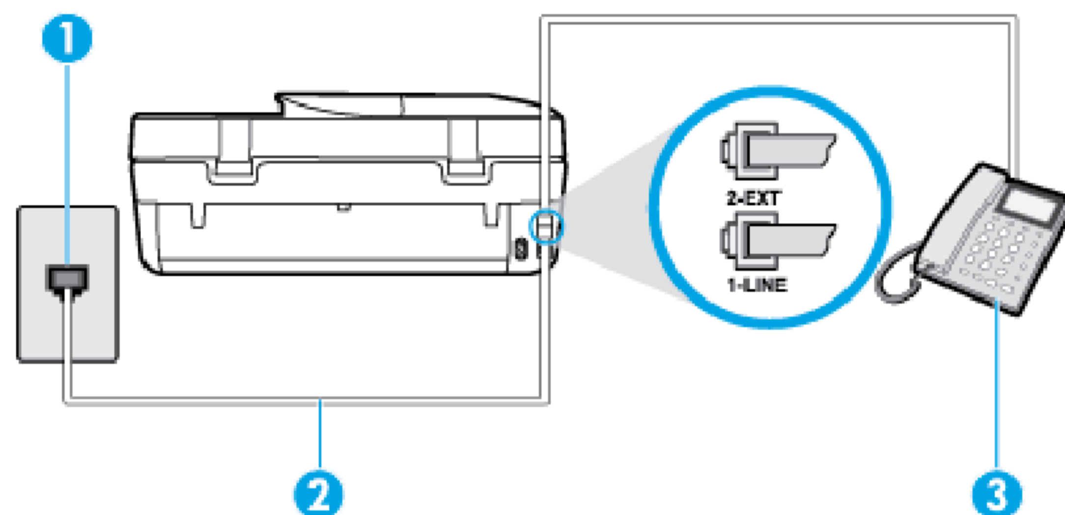
Figure B-4 Back view of the printer
