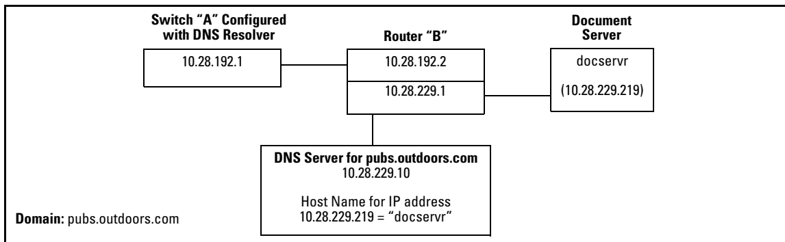
Figure C-29. Example Network Domain
