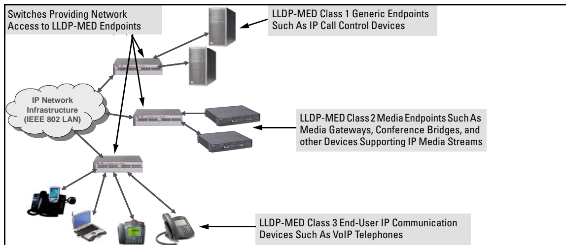
Figure 13-17. Example of LLDP-MED Network Elements
