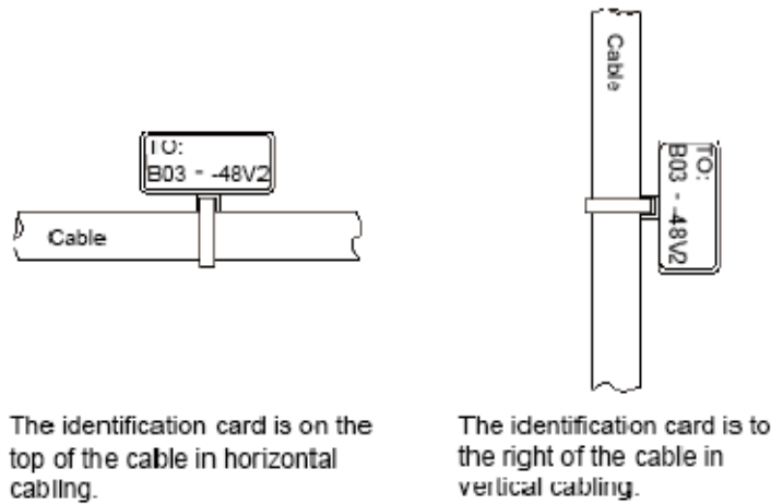
Figure 5-87 Binding the label for the power cable
