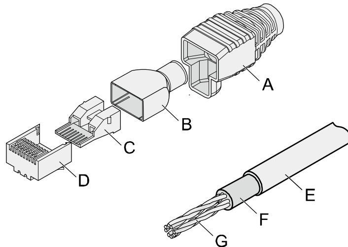
Figure 5-15 Shielded RJ45 connector and cable
