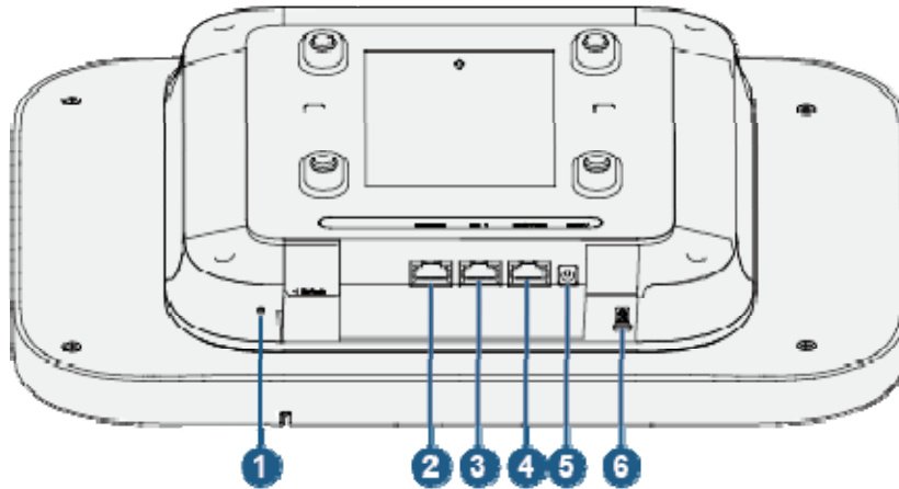
Figure 1-1 Appearance of the AP4050DN-HD
