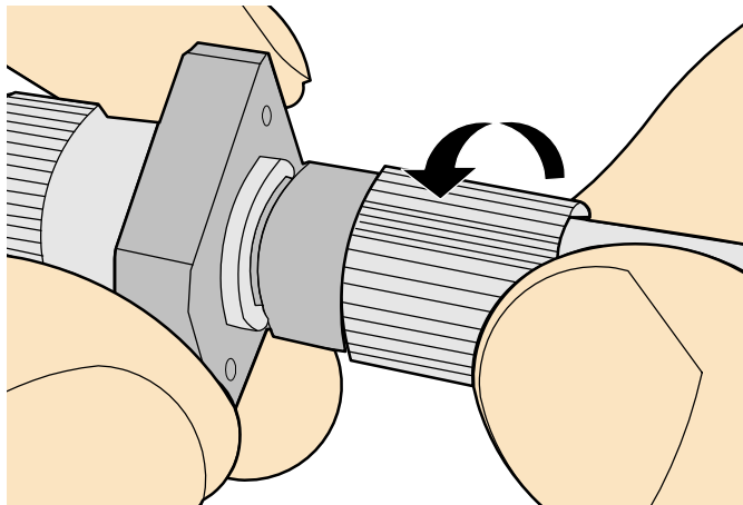
Figure 5-61 Disassembling an FC fiber connector
