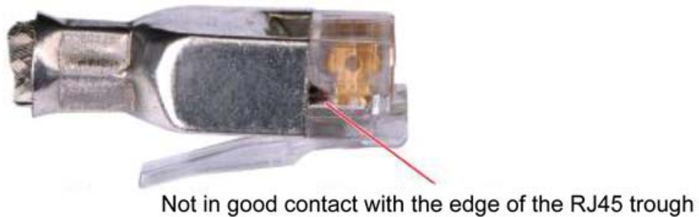
Figure 5-37 Wires not in good contact with the edge of the RJ45
