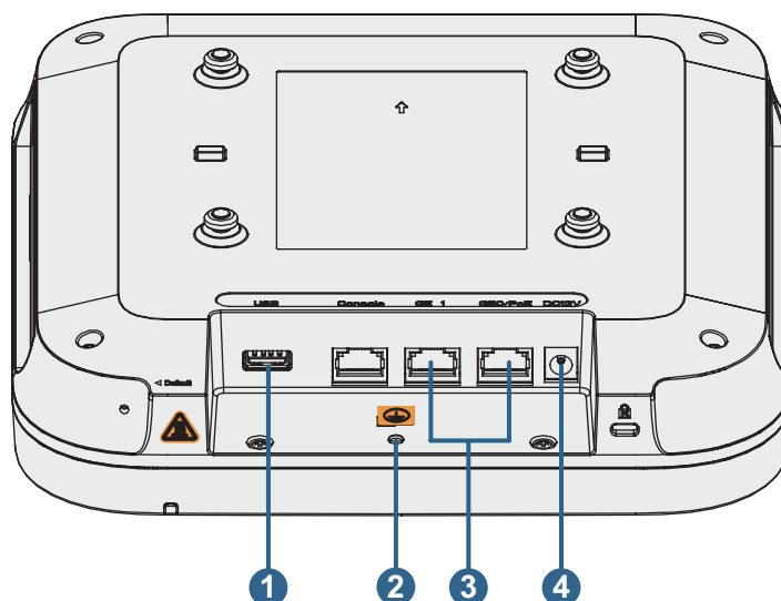
Figure 2-3 Appearance of the AP7050DE
