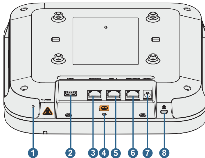
Figure 1-1 Appearance of the AP7050DE
