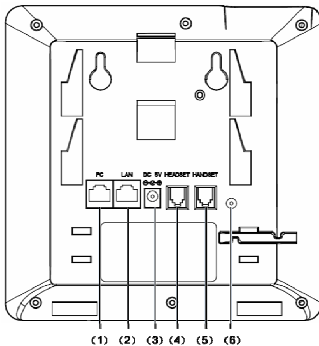
Figure 3-1 Connecting the eSpace 6805
