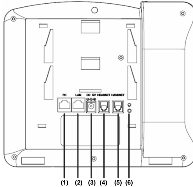
Figure 3-1 Connecting the eSpace 6830
