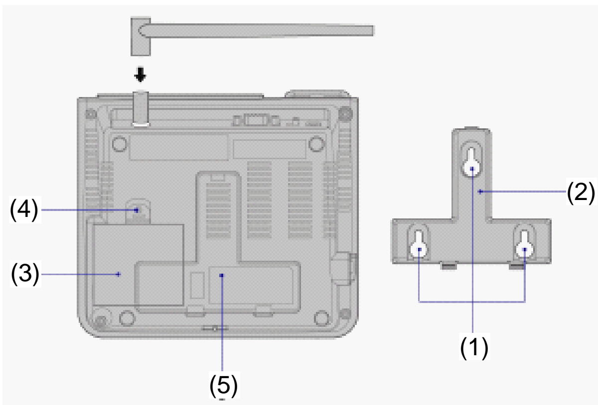
1) Hook 2) Wall-mounting bracket 3) Spare battery case 4) Tapping screw installation hole 5) Wall-mounting bracket installation area Figure 3-2 FWT back view (1)
