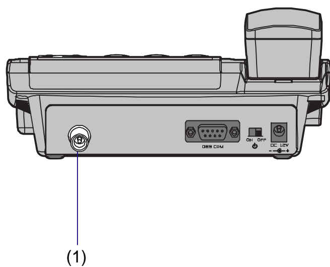
1) Installation interface to indoor antenna Figure 3-5 FWT side view (2)
