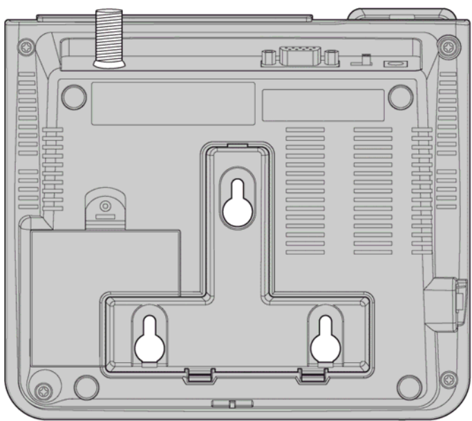
Figure 4-8 Wall-mounting bracket installation
