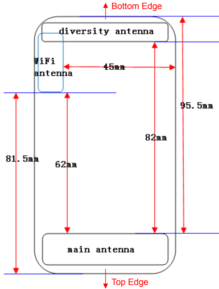
c: Antenna Schemes
