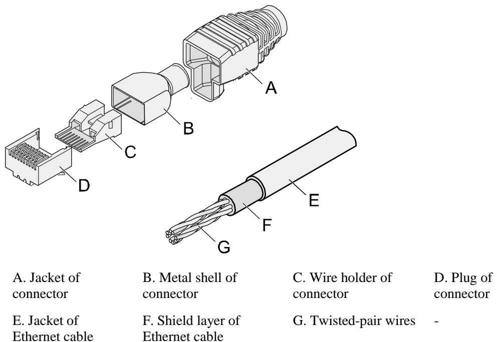
Figure 5-15 Shielded RJ45 connector and cable
