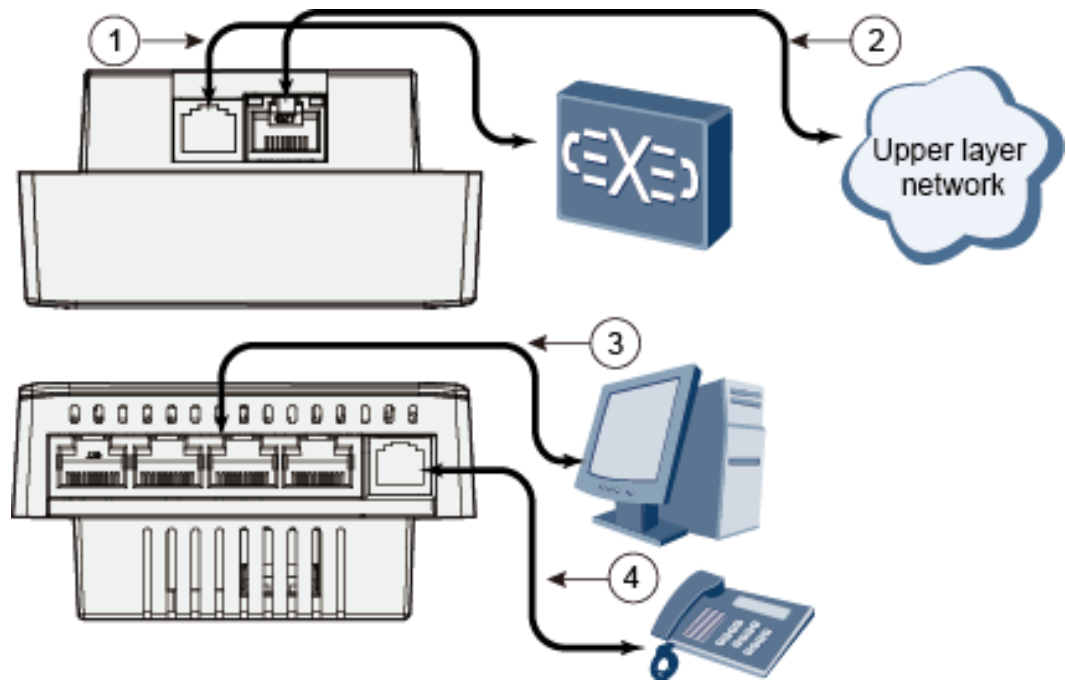
Figure 2-3 Interfaces of the R240D
