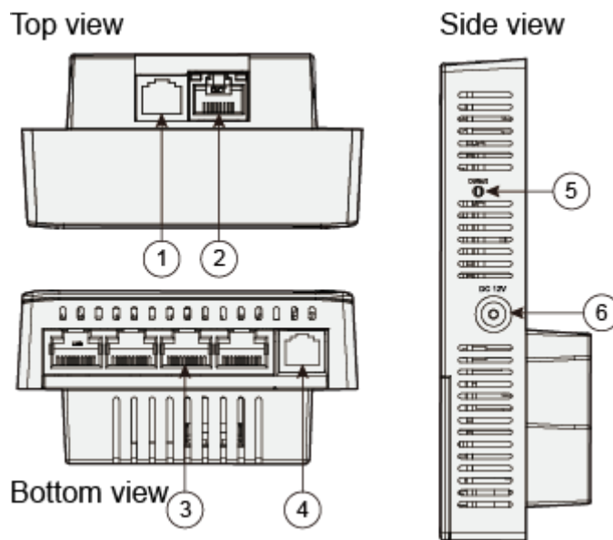
Figure 1-1 Appearance of the R240D
