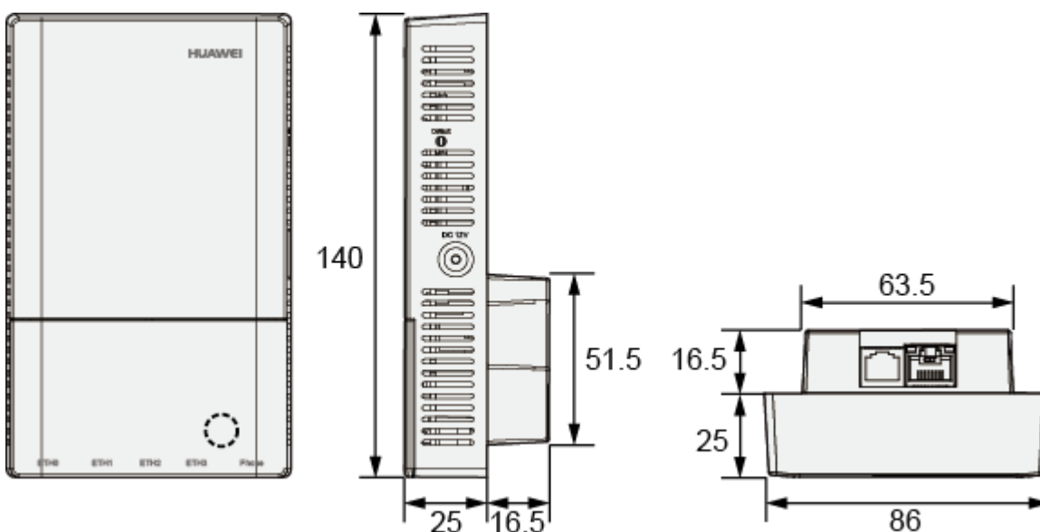
Figure 2-2 Dimensions of the R240D (unit: mm)
