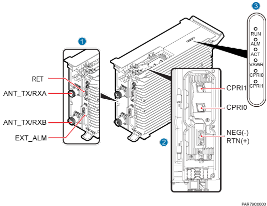
Figure 3-4 Ports on the RRU panels
