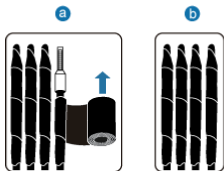
Figure 7-21 Method for handling cord end terminals that are not in use
