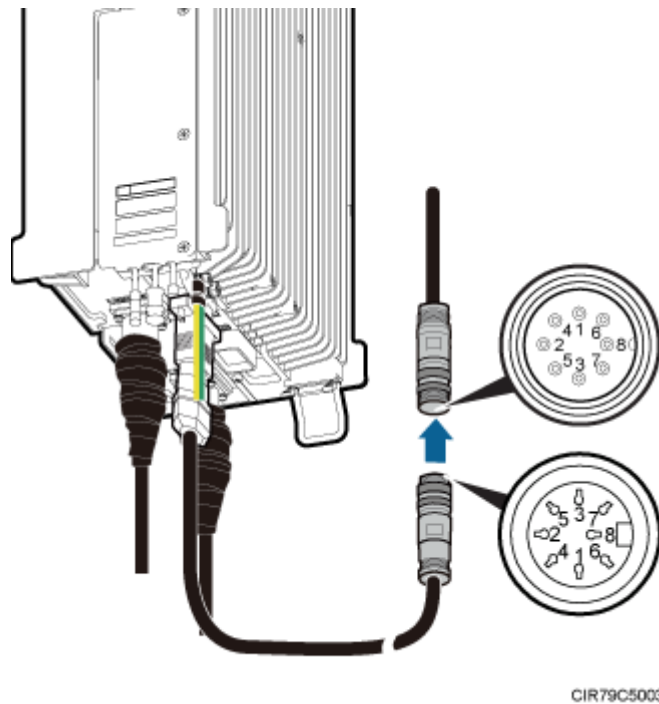
Figure 7-18 Installing an RRU AISG multi-wire cable
