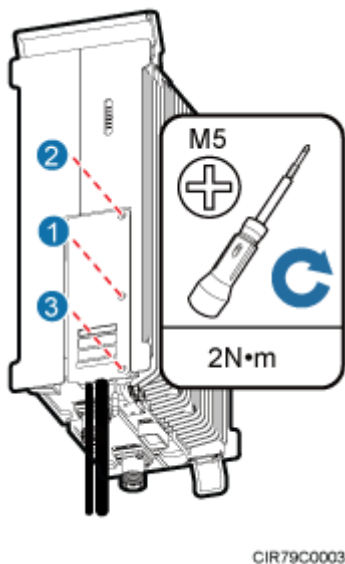
Figure 7-29 Closing the cover plate of an RRU cabling cavity
