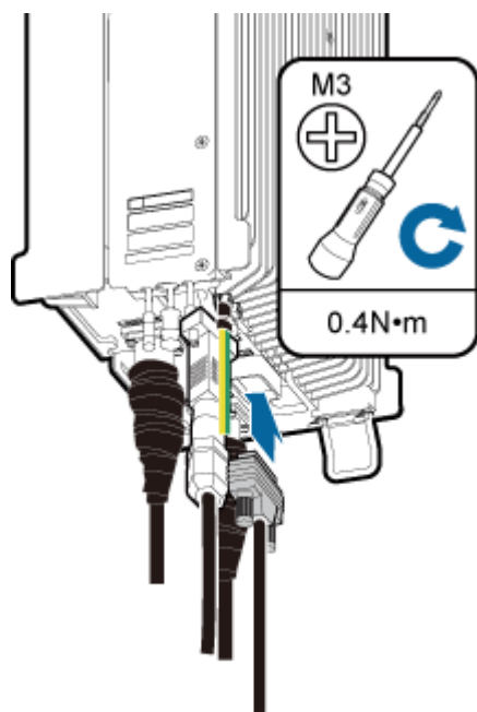
Figure 7-20 Installing an RRU alarm cable
