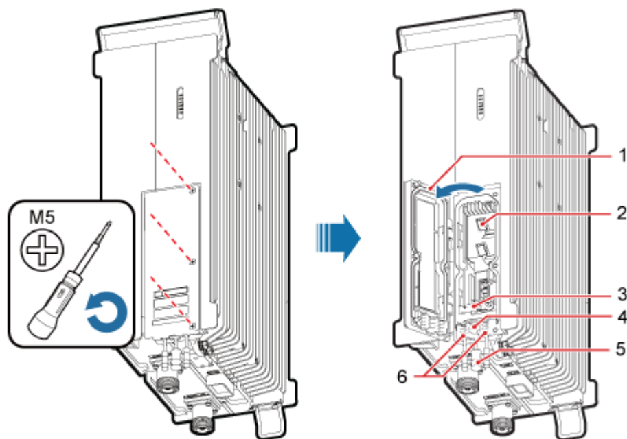
Figure 7-22 Opening the cover plate of the RRU cabling cavity
