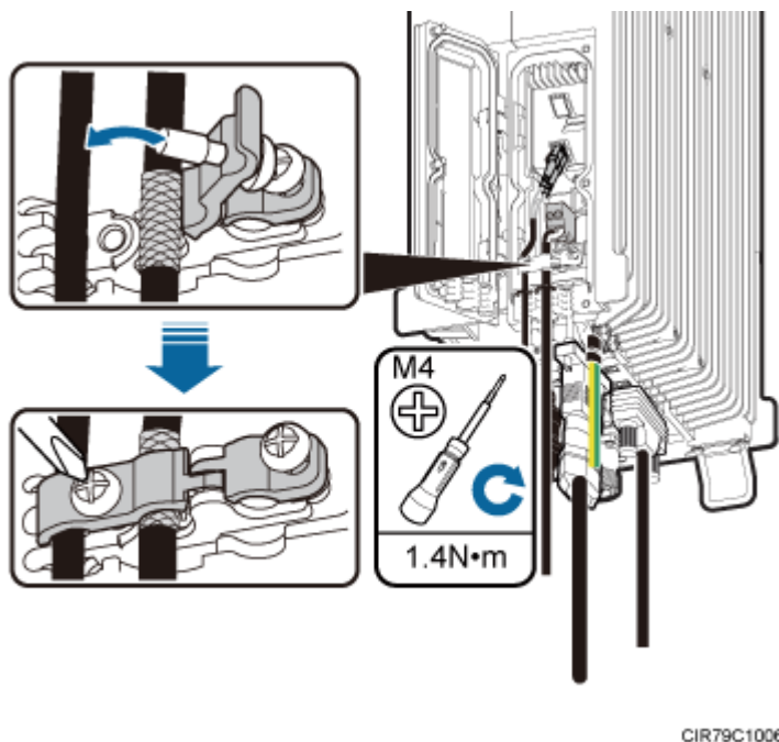
Figure 7-27 Closing clips
