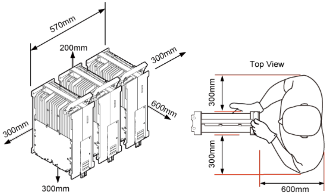
Figure 3-10 Minimum installation clearance for multiple RRUs installed in centralized mode
