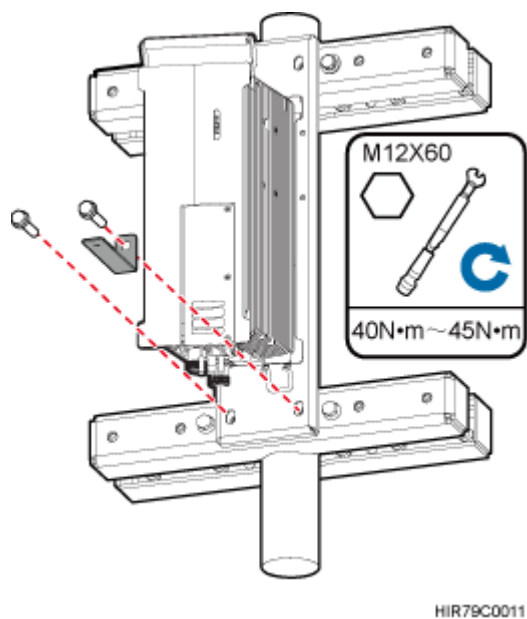
Figure 6-16 Installing the backplane and the L plate on the lower mounting bracket
