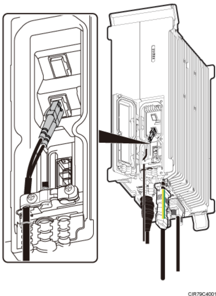
Figure 7-25 Installing a CPRI optical cable
