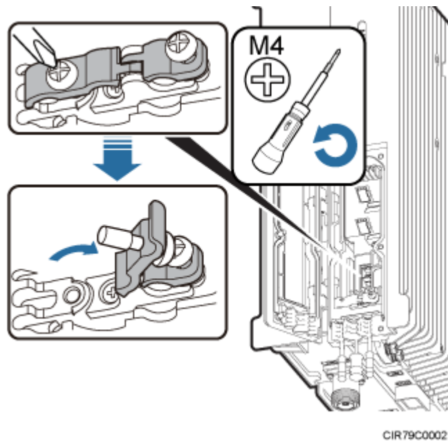
Figure 7-23 Opening clips
