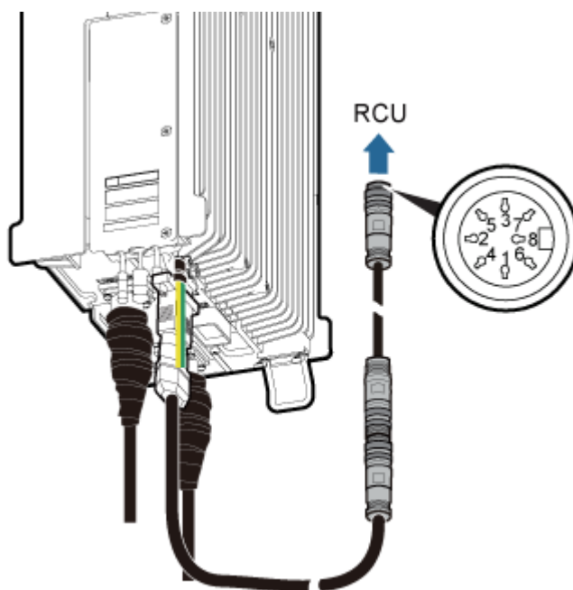
Figure 7-19 Installing an RRU AISG extension cable
