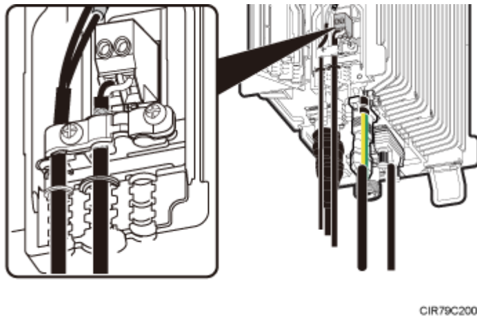
Figure 7-26 Installing an RRU power cable
