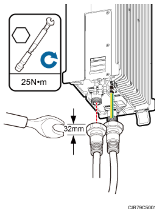
Figure 7-14 Installing an RRU RF jumper
