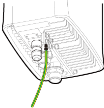
Figure 14-4 Connecting the PGND cable for the RRU to the wiring terminal at the bottom
