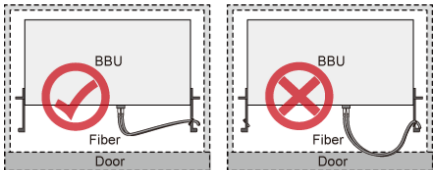
Figure 8-6 FE/GE cables routed through the cabinet
