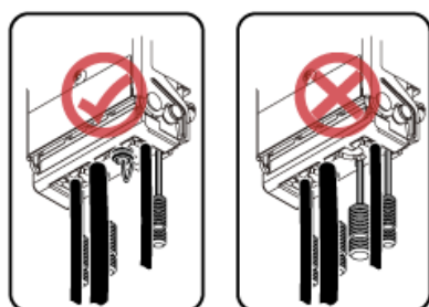
Figure 8-29 Correct placement of waterproof blocks
