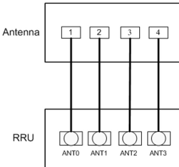
Figure 8-14 The mapping relationship between the RF ports and the antenna ports
