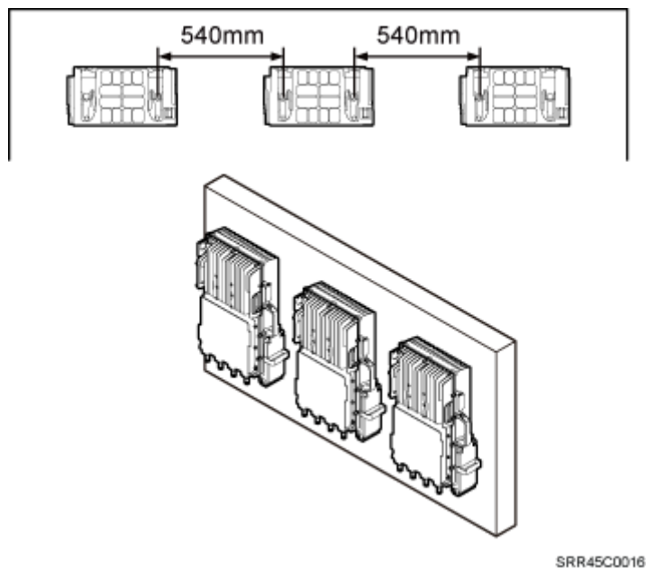
Figure 3-18 Minimum clearance for multiple RRUs installed on a wall in standard mode
