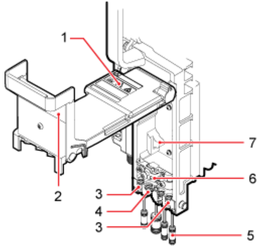
Figure 8-23 RRU cabling cavity
