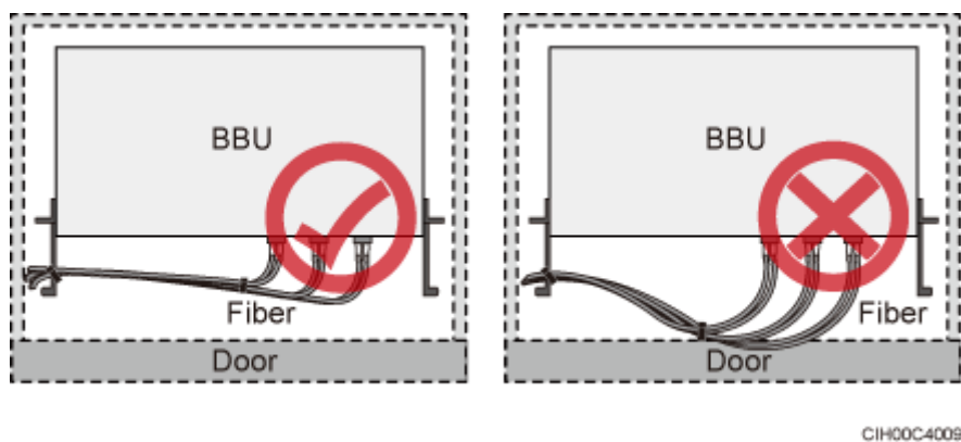
Figure 8-5 CPRI fiber optic cables routed through the cabinet (2)
