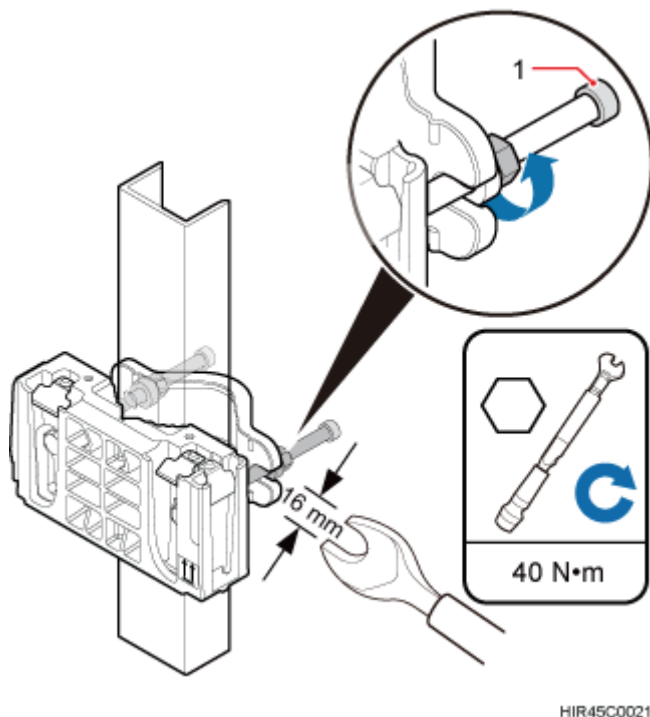
Figure 7-27 Securing the bracket assembly
