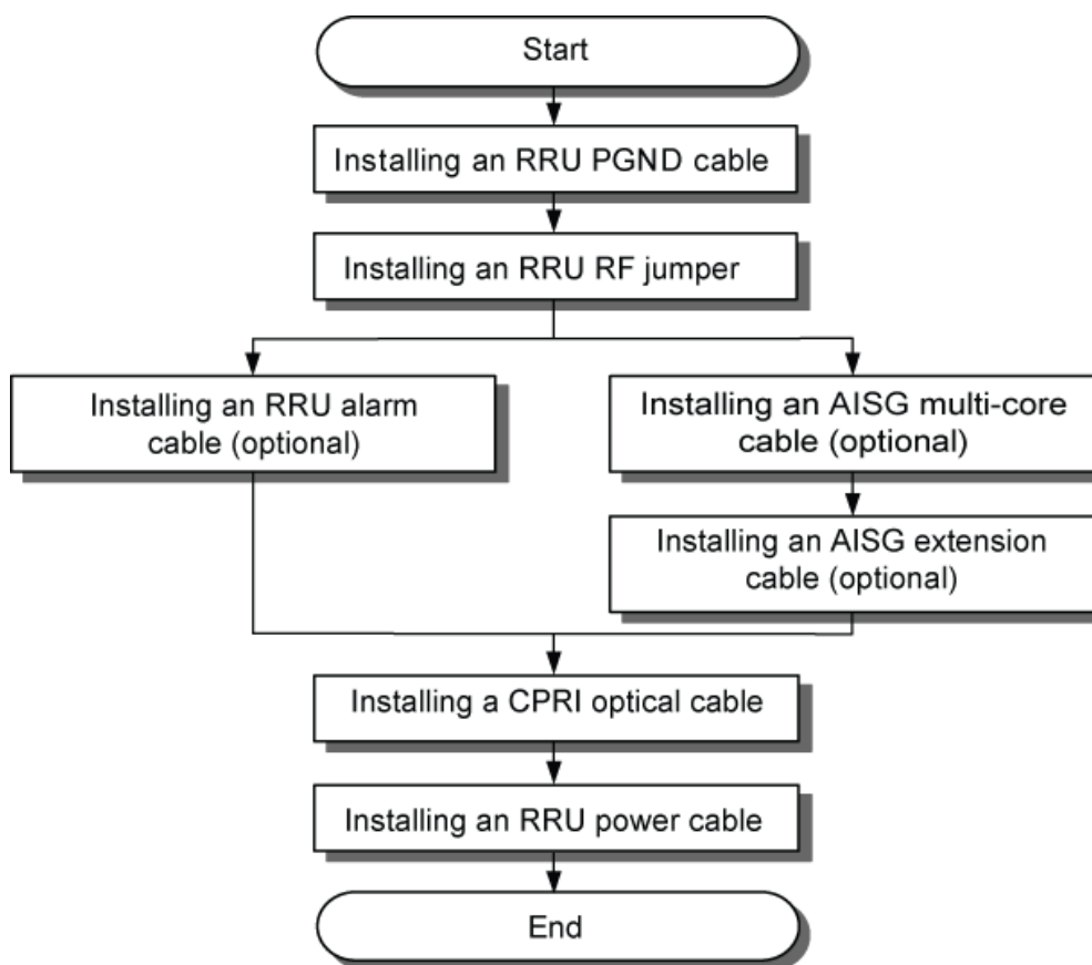
Figure 8-11 Process of installing RRU cables
