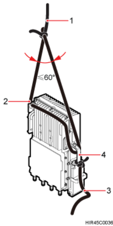
Figure 6-3 Binding the RRU
