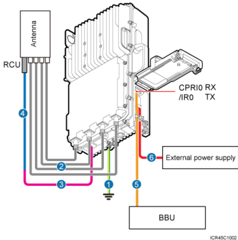
Figure 8-8 Cable connections for a single RRU (2)
