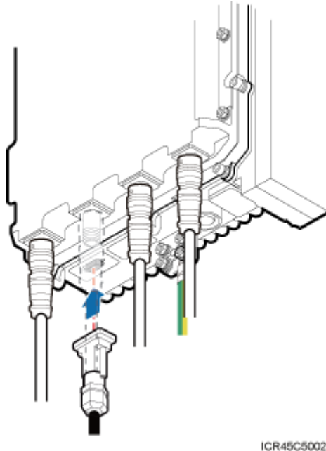
Figure 8-19 Installing an RRU AISG multi-wire cable
