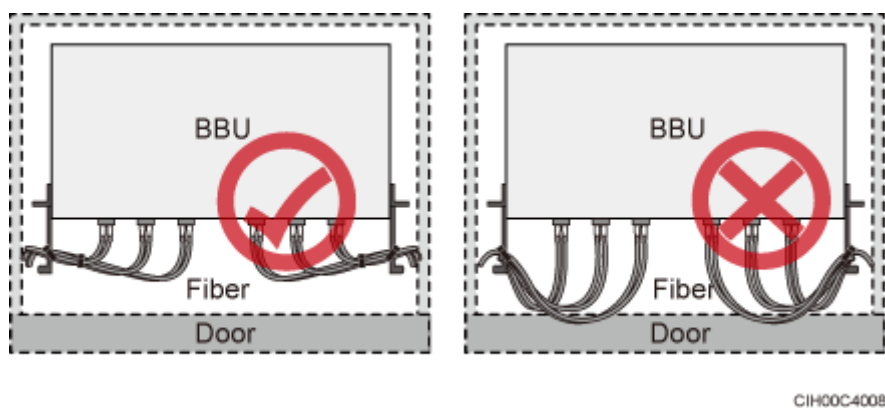
Figure 8-4 CPRI fiber optic cables routed through the cabinet (1)
