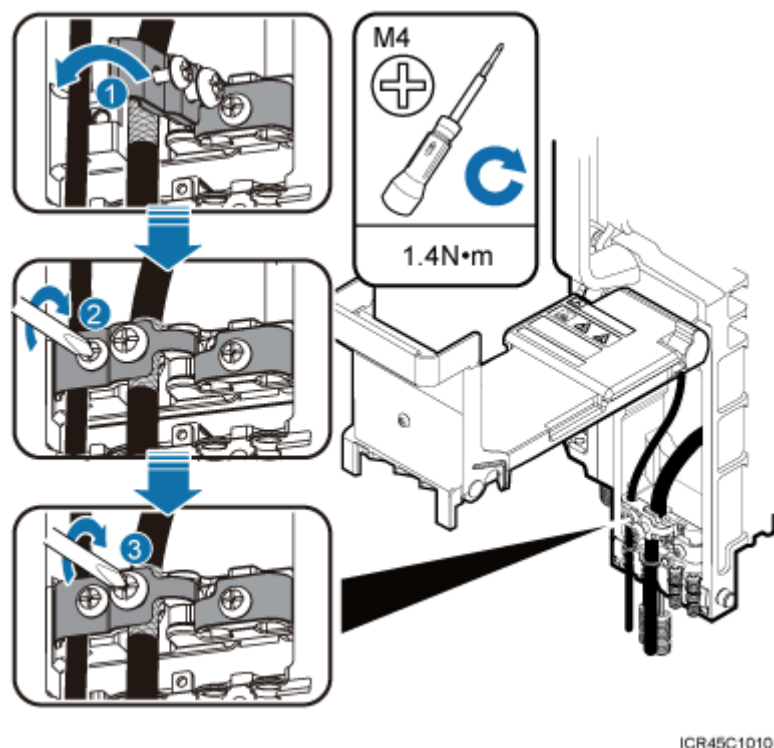
Figure 8-28 Closing clips
