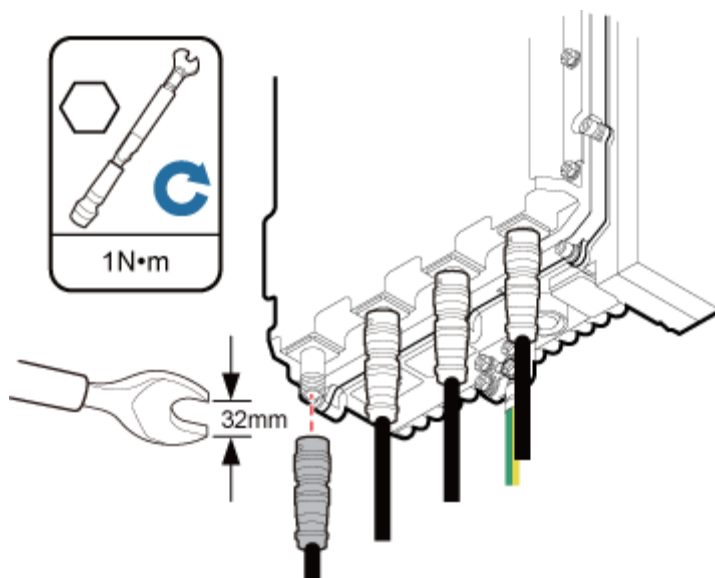
Figure 8-15 Installing an RRU RF jumper
