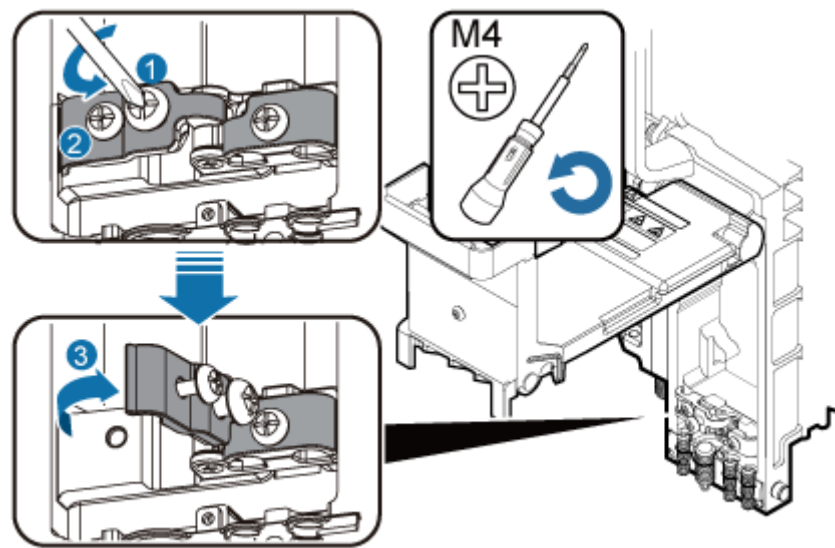
Figure 8-24 Opening clips
