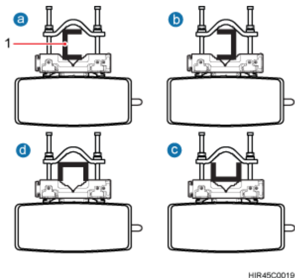
Figure 7-23 Top view of the RRU
