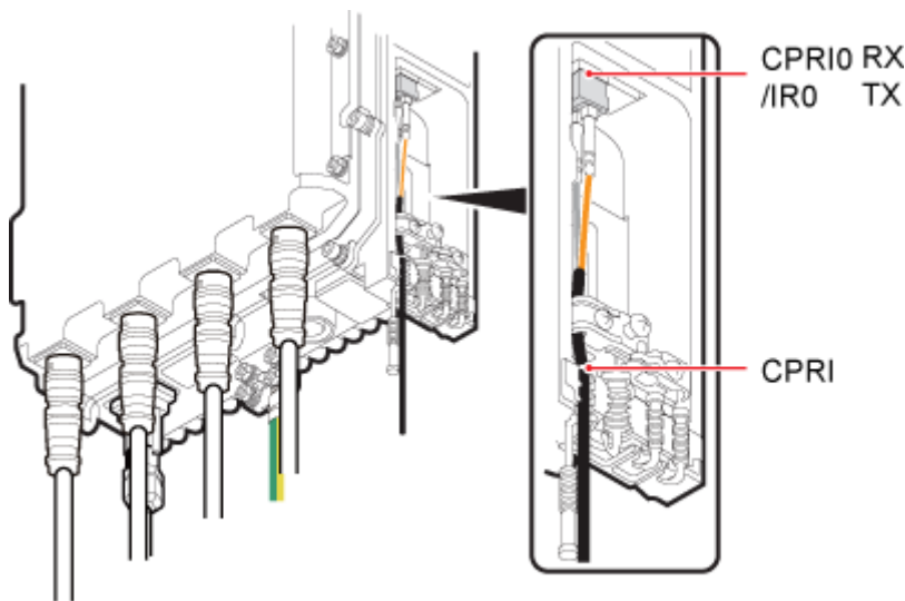
Figure 8-27 Installing a CPRI optical fiber cable
