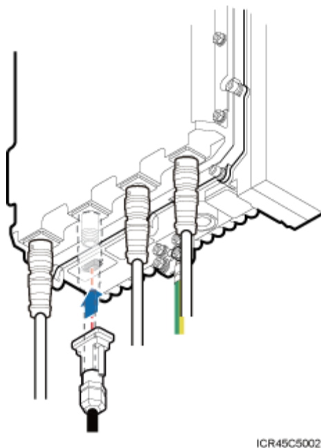
Figure 8-18 Installing an RRU alarm cable
