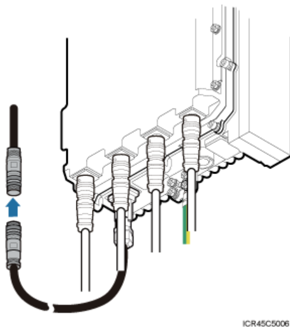
Figure 8-20 Installing an RRU AISG multi-wire cable
