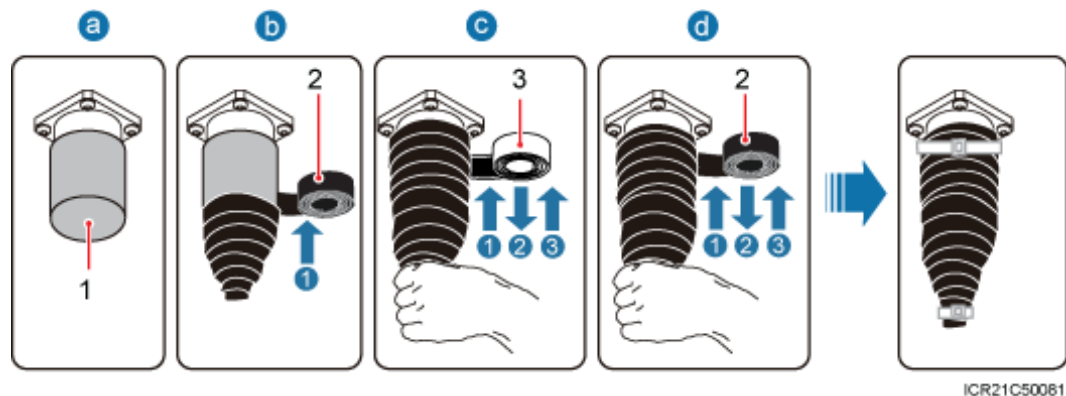
Figure 8-17 Waterproofing a dustproof cap
