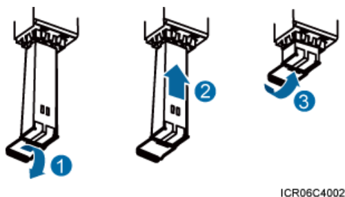
Figure 8-26 Installing an optical module
