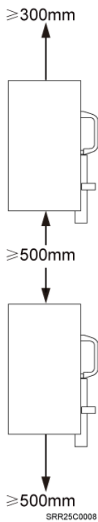
Figure 3-22 Recommended vertical spacing between RRUs
