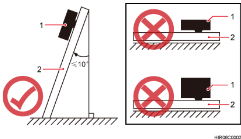
Figure 3-5 Requirement of the angle between the ground and the pole, angle steel, or U-steel
