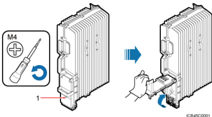
Figure 8-22 Opening the cover plate of the RRU cabling cavity
