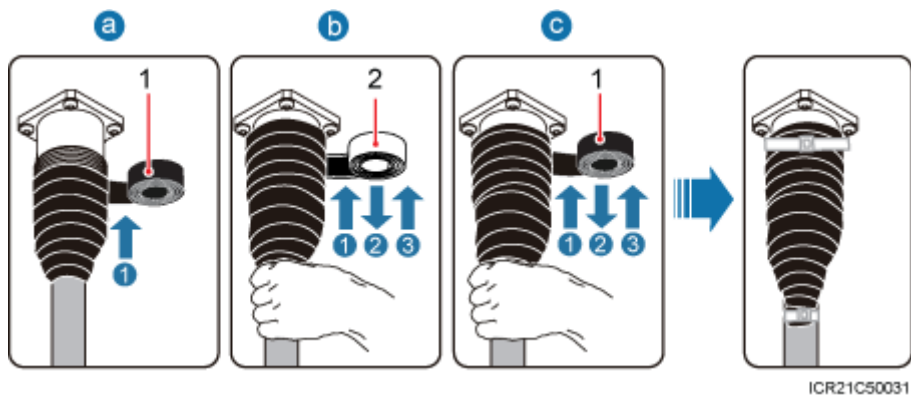
Figure 8-16 Waterproofing a connector of the RF jumper
