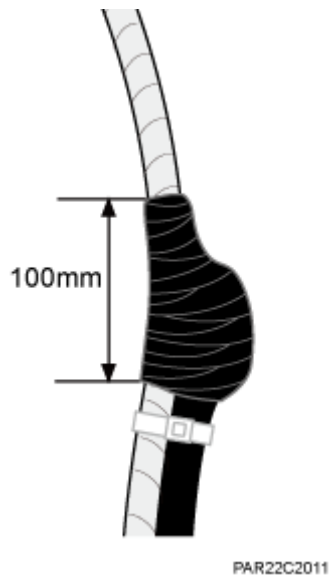
Figure 6-11 Wrapping the PVC insulation tape
