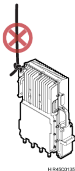
Figure 6-5 Incorrect binding method - hoisting the RRU by the lifting eye only
