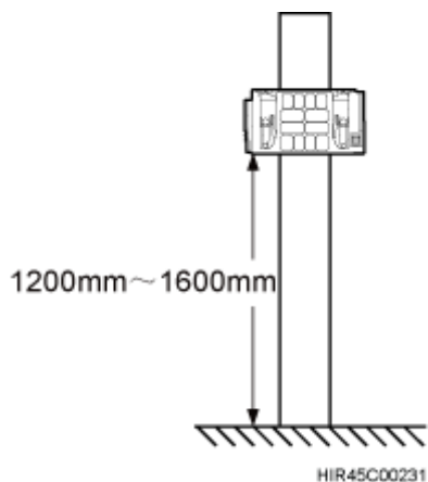
Figure 7-24 Distance between the main mounting bracket and the ground
