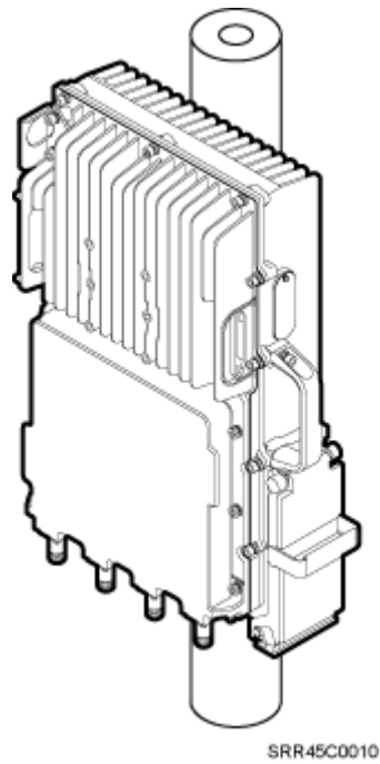
Figure 3-6 RRU installed on a pole
