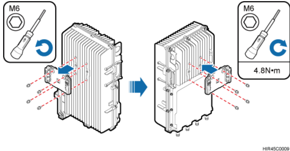
Figure 7-14 Removing the attachment plate from the rear of the second RRU and then installing it on the RRU front
