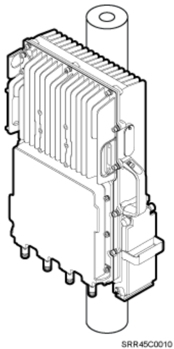
Figure 7-3 Single RRU installed on a pole
