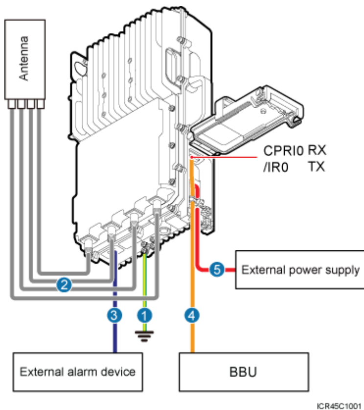
Figure 8-7 Cable connections for a single RRU (1)
