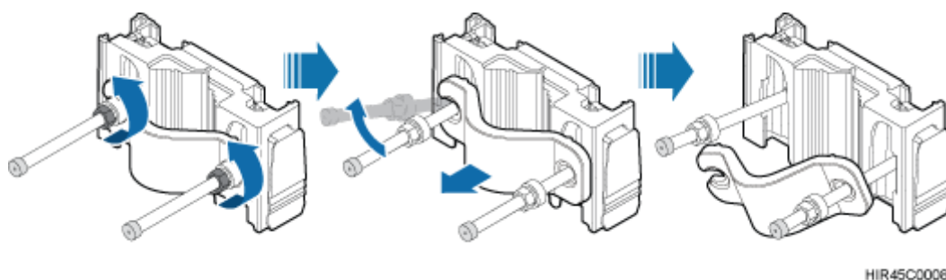
Figure 7-31 Removing the M10x150 bolt from the U notch
