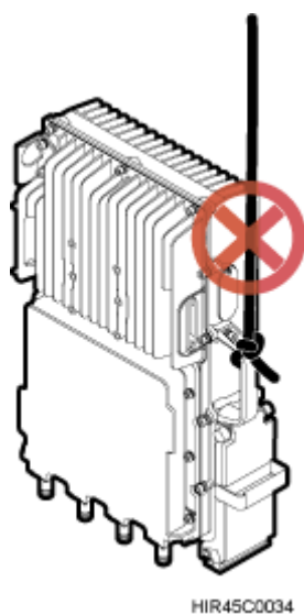
Figure 6-4 Incorrect binding method - hoisting the RRU by the handle only
