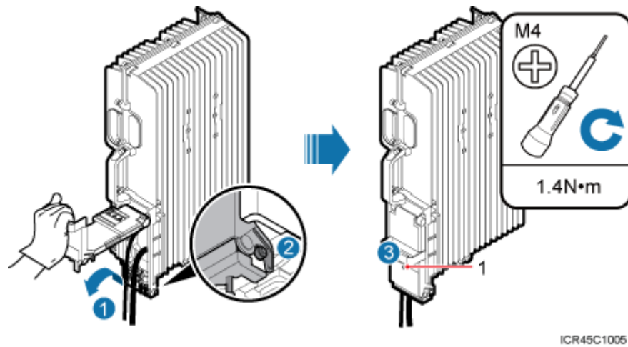
Figure 8-30 Closing the cover plate of the RRU cabling cavity
