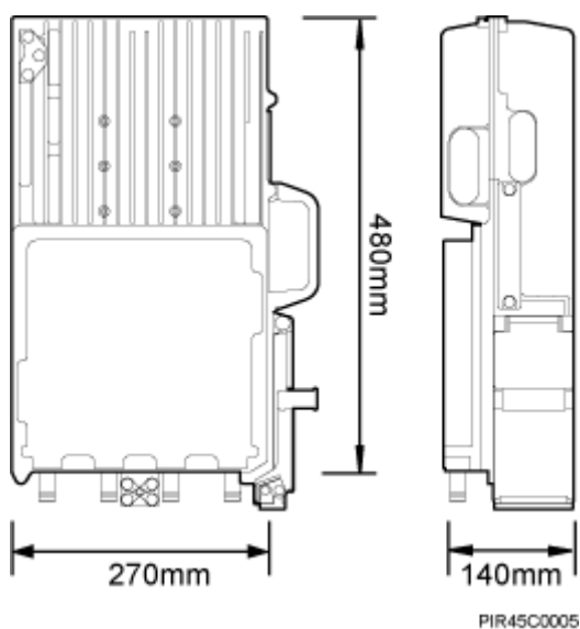
Figure 3-2 RRU dimensions
