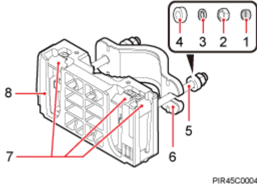
Figure 7-1 Bracket assembly for an RRU
