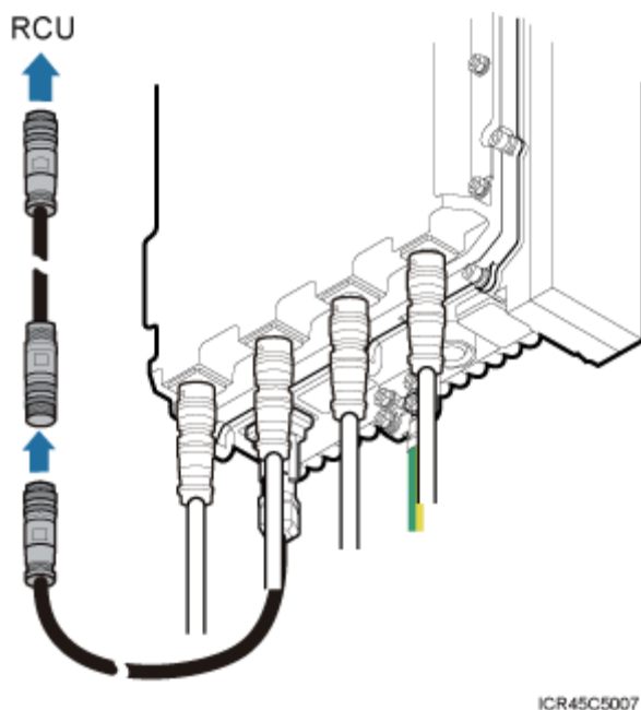
Figure 8-21 Installing an RRU AISG multi-wire cable
