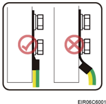
Figure 8-13 Correct direction of an OT terminal
