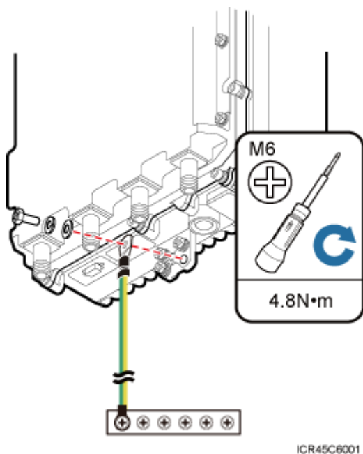
Figure 8-12 Installing an RRU PGND cable
