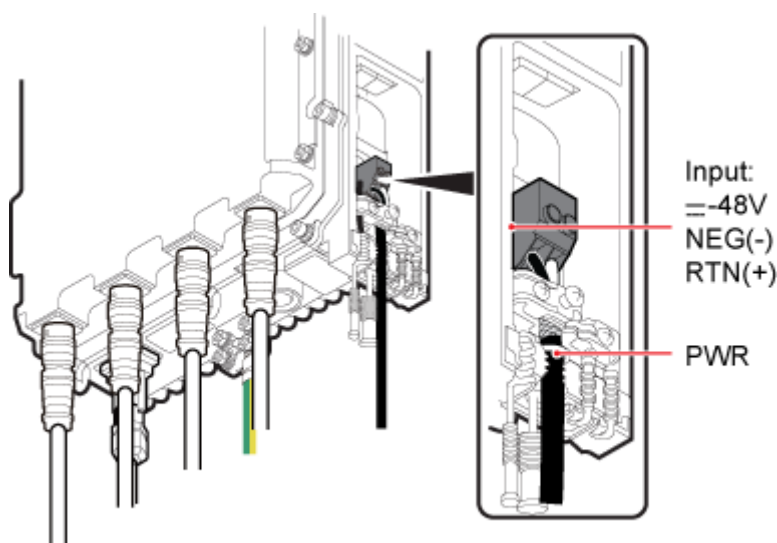
Figure 8-25 Installing an RRU power cable
