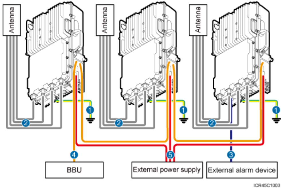
Figure 8-9 Cable connections for multiple RRUs (1)
