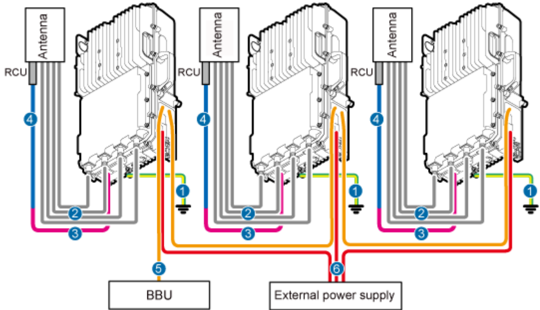
Figure 8-10 Cable connections for multiple RRUs (2)
