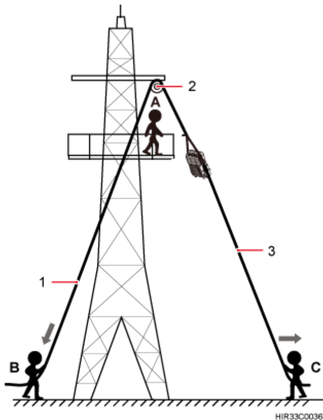
Figure 6-1 Hoisting an RRU onto a tower
