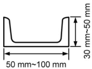
Figure 3-7 U-steel specifications
