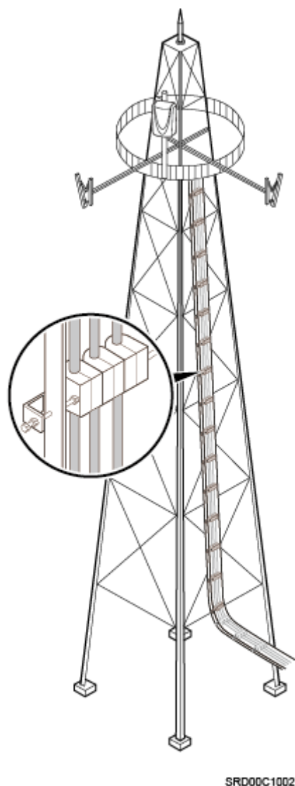
Figure 8-2 Securing cables on the tower
