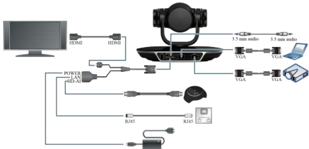
Figure 2-1 Connecting cables
