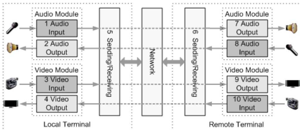
Figure 13-4 TE30 diagnostics model
