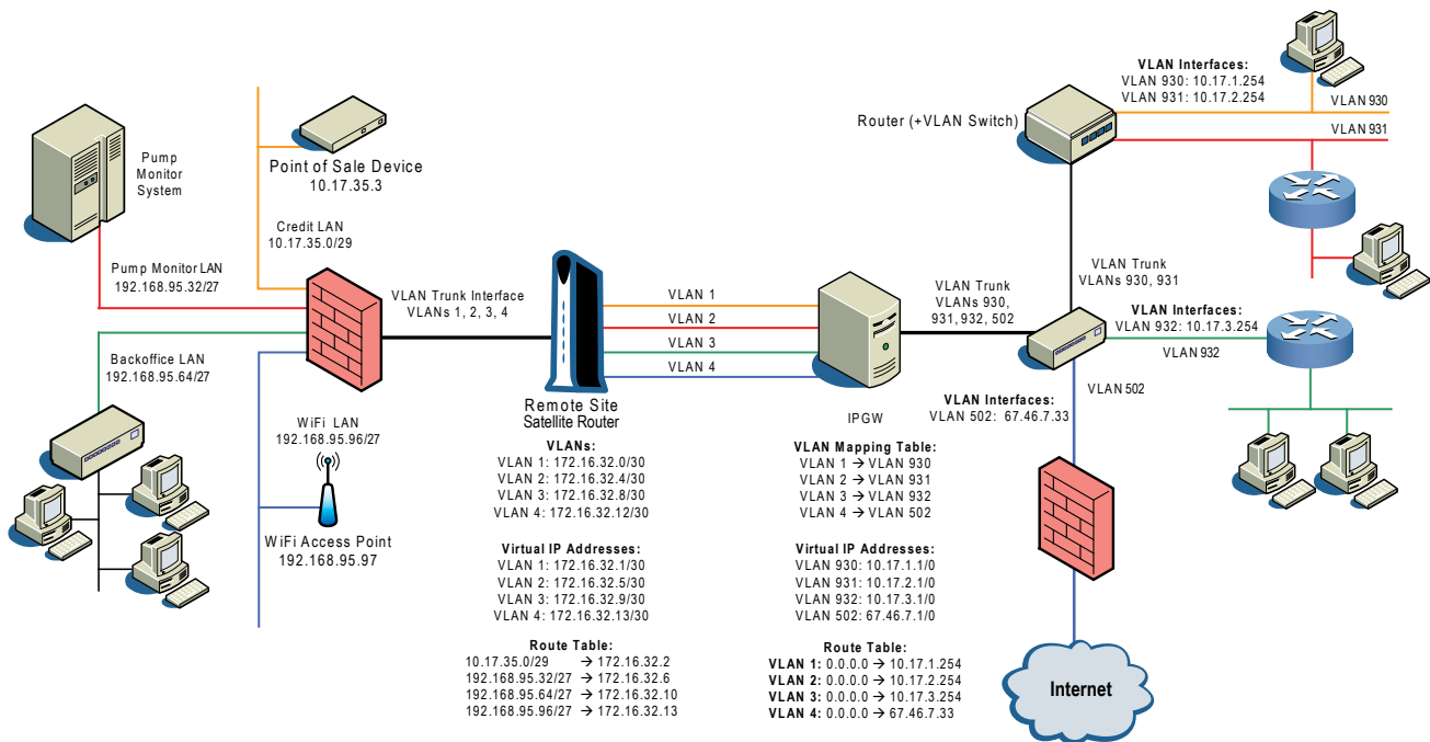
Figure 4. End-to-End VLAN Tagging Application
