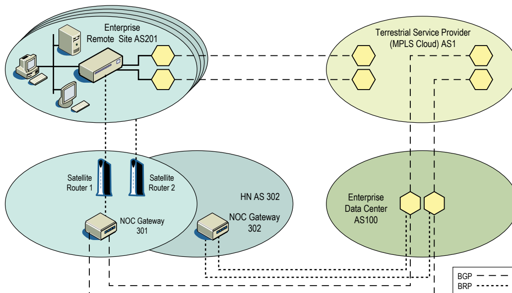
Figure 5. Use of BGP within an Intranet with Satellite
