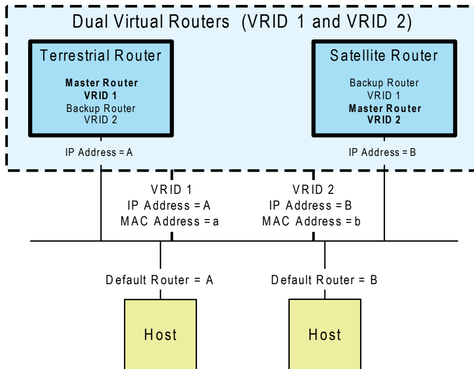
Figure 2. Dual Virtual Routers for Load Sharing
