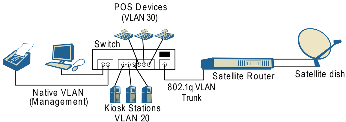
Figure 3. VLANs for Segregating Traffic
