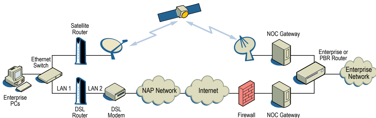
Figure 6. High Availability Network with Satellite and Terrestrial DSL Transport
