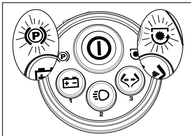
Park brake and blade switch fault lights
