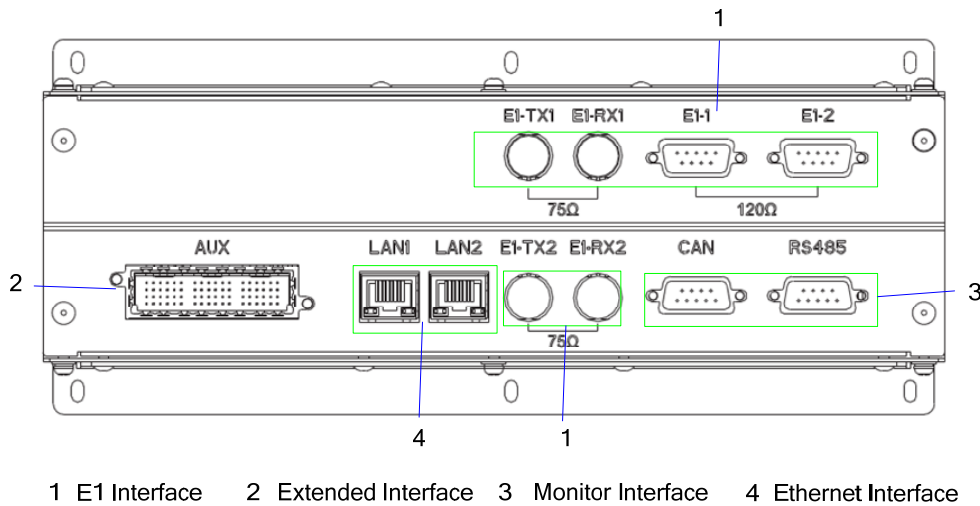
Figure 2-3 Extended Interface Board
