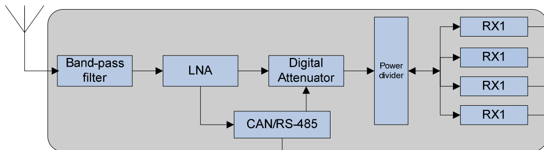
Figure 2-15 Diagram of DIU
