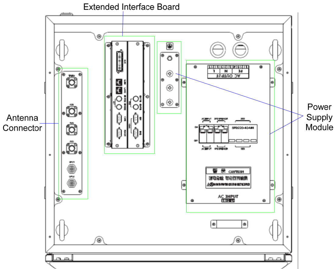
Figure 2-1 Components of Base Station Interface Unit
