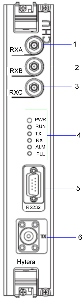
Figure 2-7 Front Panel of CHU
