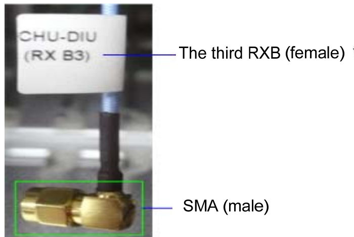
Figure 3-16 Cable Diagram
