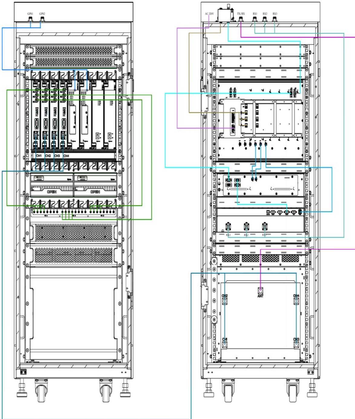
Figure 3-1 Cable Layout
